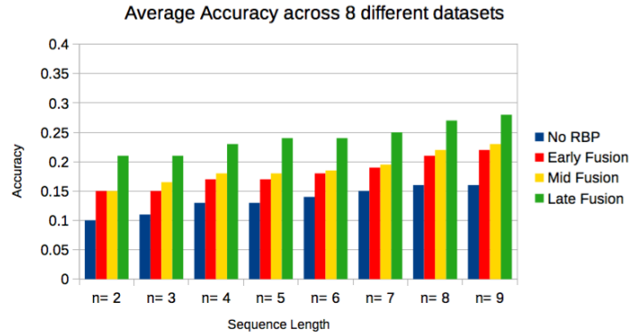
Fig. 4.12 Overall Accuracy with and without RBP across 8 datasets using RNNs for various context lengths n with integer encoding.
