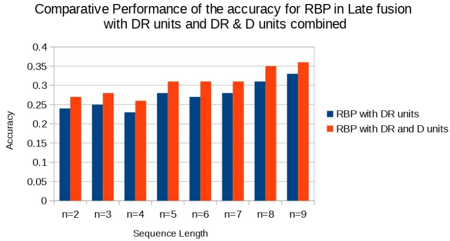
Fig. 4.17 Overall Accuracy for RBP in Late Fusion with DR units and combining DR and D units.
