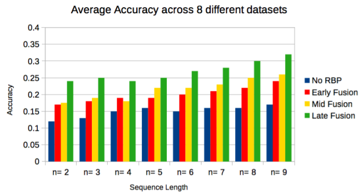
Fig. 4.13 Overall Accuracy with and without RBP across 8 datasets using GRUs for various context lengths n with integer encoding.
