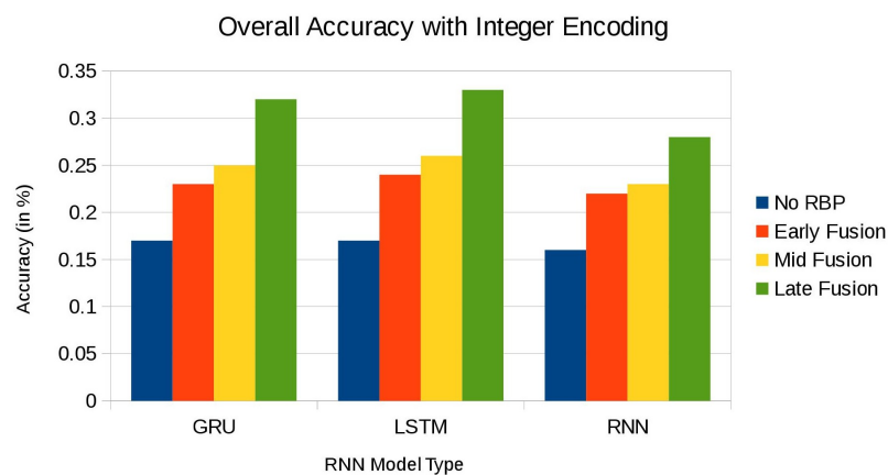
Fig. 4.10 Overall Accuracy with Integer Encoding for sequence length : 9 without RBP and RBP in Early, Mid and Late Fusion.
