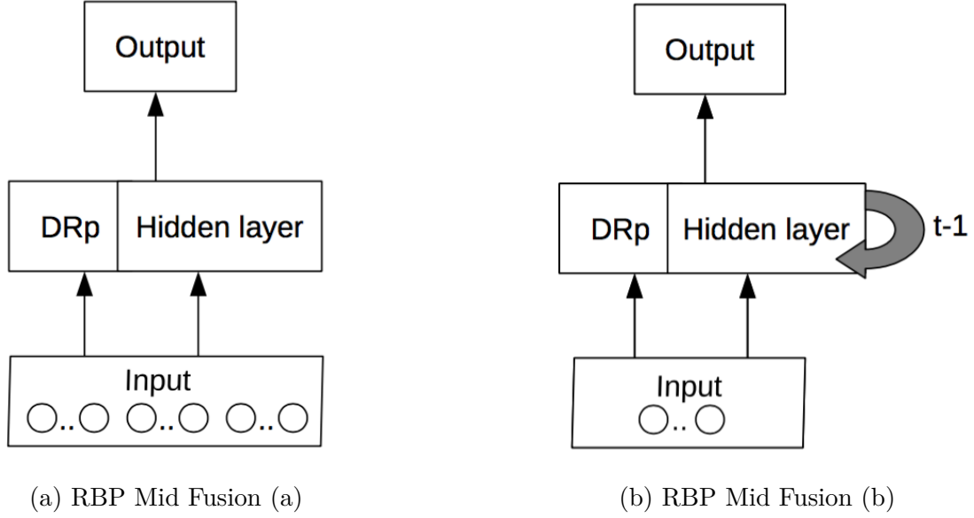
Fig. 3.4 Overview of RBP Mid Fusion approaches, where the DR_{pout} units are concatenated to the hidden layer. In the case of recurrent network, an additional context from the previous layer is there, the rest of the network is the same as shown in (a) where DR_p units are added to the first hidden layer. DR_p units are calculated using the tokens in the input layer. The only difference from Early Fusion is that here the DR_p are added to the hidden layer unlike previously where they are added to the input layer.
