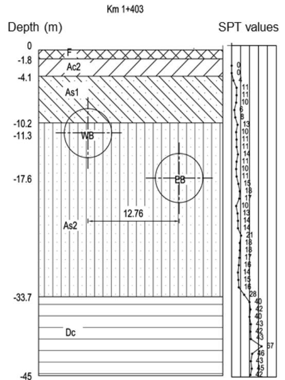
Figure 4. Tunnel arrangement and geotechnical profiles (Le et al. 2019b).
