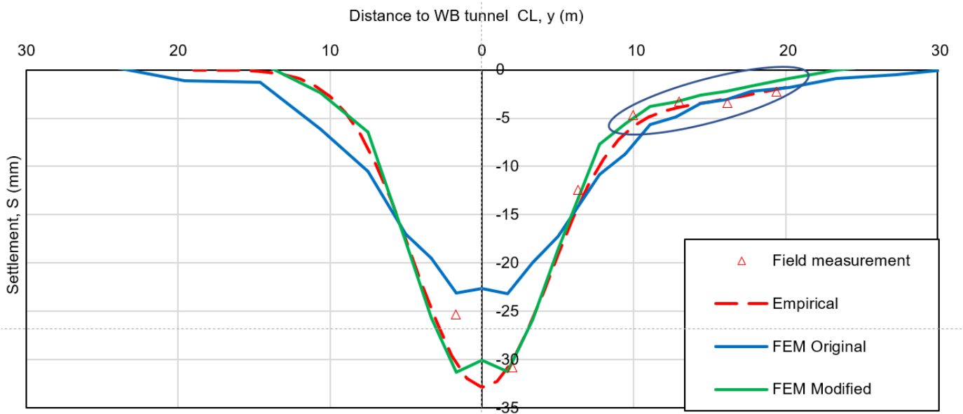
Figure 8. Ground surface settlement after WB tunnel construction.
