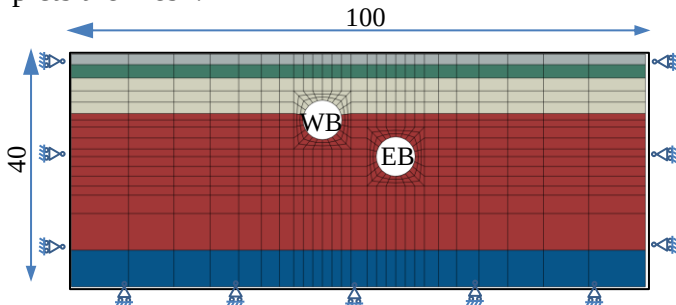
Figure 5. Finite element model in Abaqus.
