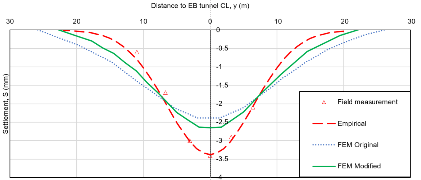
Figure 7. Ground surface settlement after EB tunnel construction.
