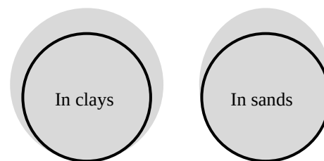
Figure 2. Typical ground loss distribution for shallow tunnels (after Franza et al. 2019).
