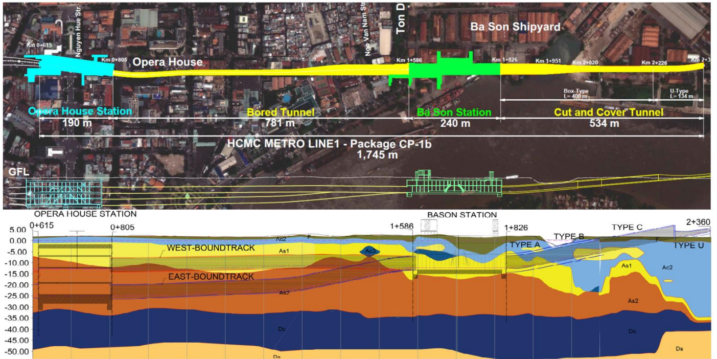
Figure 3. The underground section of line Ben Thanh – Suoi Tien (Kuriki 2008).
