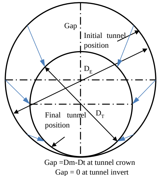
Figure 1. The gap method (After Potts & Zdravkovic 2001).
