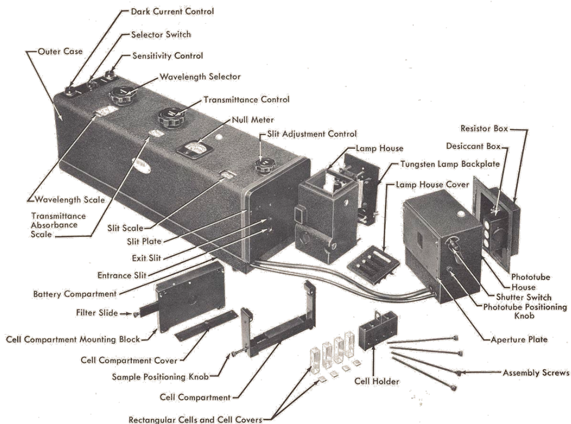
Figure 3.6: Beckman DU Spectrophotometer (Picture from the archives Beckman Historical Collection ) 144 .
