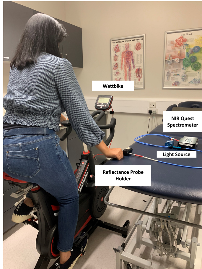
Figure 9.1: Set-up of the in-vivo experiments where a volunteer was recruited for an incremental exercise bike study and NIR spectra was collected from the thumb using a portable NIR spectrometer, NIR Quest, a light source and a reflectance probe holder.
