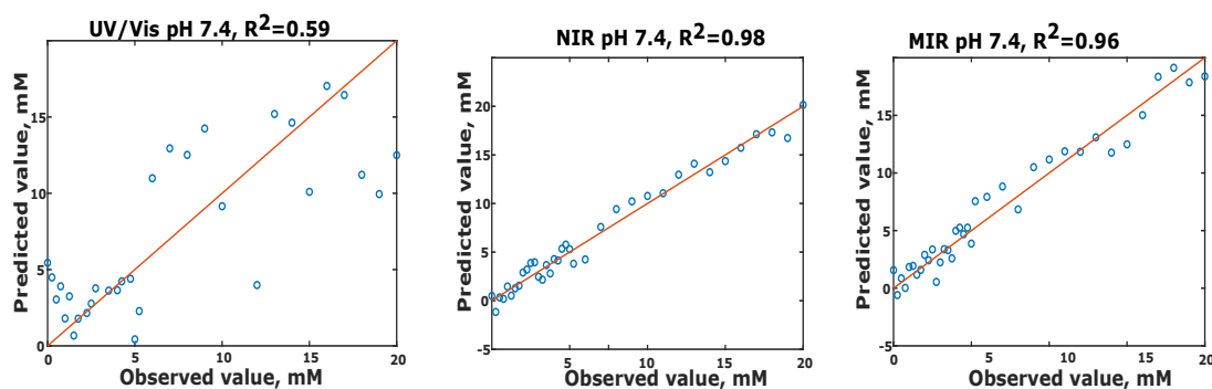
Figure 5.9: Observed (known) lactate concentration versus the Predicted concentrations of thirty-seven PBS samples of lactate prepared using solution stoichiometry. The correlation coefficient ( R^2 ) and the root mean squared error of cross validation (RMSECV) for each set are also shown. (a) The Coefficient of Determination ( R^2 ) and the root mean squared error of cross validation (RMSECV) for UV/Vis set is 0.59 and 4.27 mM respectively; (b) The Coefficient of Determination ( R^2 ) and the root mean squared error of cross validation (RMSECV) for NIR set is 0.98 and 0.89 mM respectively; (c) The Coefficient of Determination ( R^2 ) and the root mean squared error of cross validation (RMSECV) for MIR (FTIR) set is 0.96 and 1.16 mM respectively.
