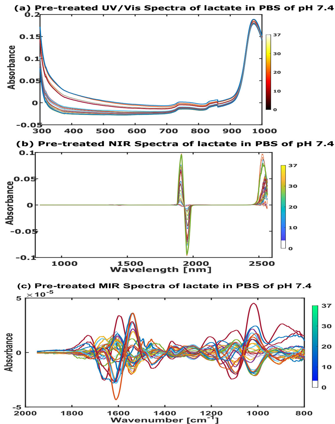
Figure 5.3: Pre-treated spectra of the UV/Vis, NIR and MIR (FTIR) of all the samples after pre-processing; subtraction of base sample (0.25 mM of lactate concentration), Extended Mean Signal Correction (EMSC) and Savitzk-Golay (SG) derivation. (a) 36 pre treated spectra in the UV/Vis spectral region; (b) 36 pre treated spectra in the NIR spectral region; (c) 36 pre treated spectra in the MIR region.
