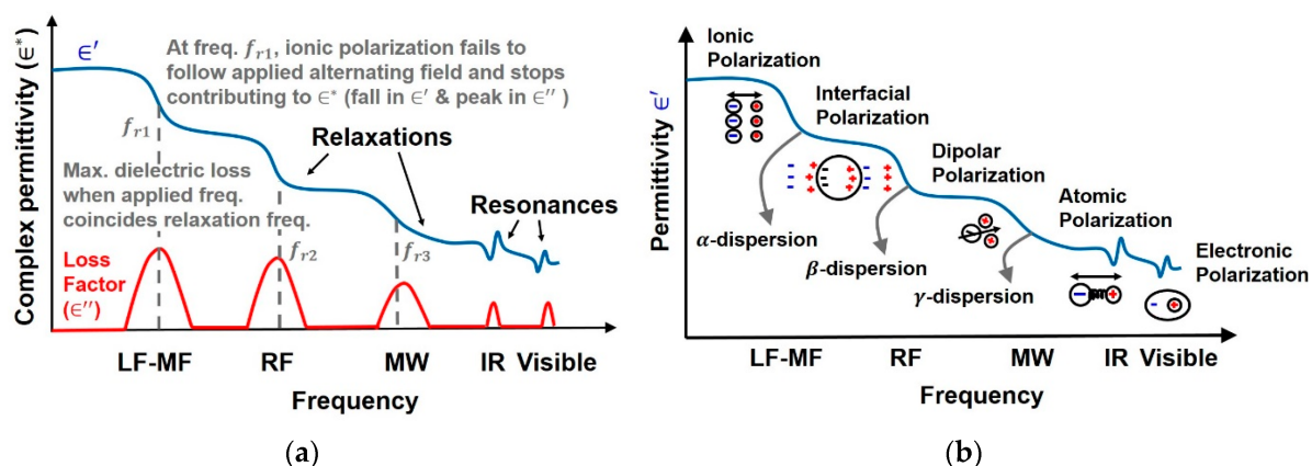
Figure 4.6: The picture depicts the behavior of a medium in the following parts of the Electromagnetic Spectrum: LF-MF: Low and Medium Frequency, RF: Radio Frequency, MW: Microwave, IR: Infrared and Visible, when an increasing frequency alternating field is applied. (a) The behaviour when the medium is a dielectric. Relaxations are noted in the Radio Frequency and Microwave frequencies, whereas, resonances in the Infrared and Visible frequencies. These relaxation frequency shifts occur due to change in permittivity of a material. (b) Polarization and relaxation shifts are also seen in these frequency ranges as ionic, followed by interfacial, dipolar, atomic and electronic. Picture taken from 212 .
