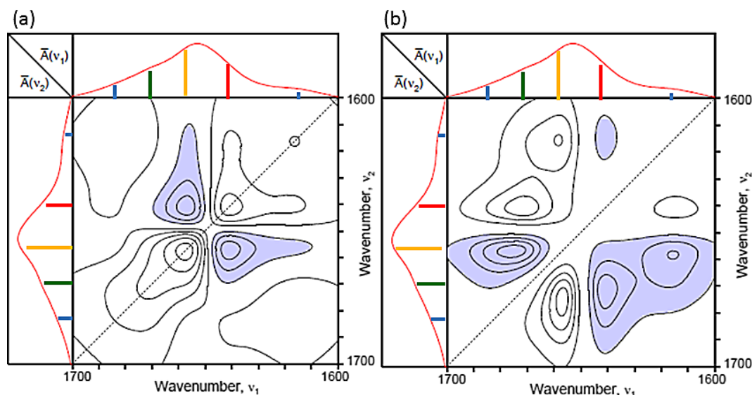
Figure 3.11: An example of (a) Synchronous and (b) Asynchronous 2D correlation spectrum. Picture taken from 161 .
