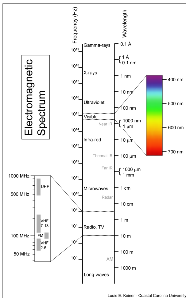
Figure 3.1: The Electromagnetic Spectrum (EM) depicting the various regions like Gamma-rays, X-rays, Ultraviolet (UV), Visible (Vis), Infrared, Microwaves, Radio, TV and Long-waves based on the frequency (Hz), \nu and wavelength (length-scale), \lambda . The visible region is highlighted (400-700 nm ). Figure taken from 133 .
