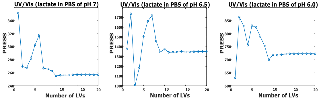
Figure 6.4: Prediction Error Sum of Squares (PRESS) versus number of latent variables (LV). (a) The number of LVs in the UV/Vis spectral region for pH 7 used was 3; (b) The number of LVs in the UV/Vis spectral region for pH 6.5 used was 3; (c) The number of LVs in the UV/Vis spectral region for pH 6 used was 4.
