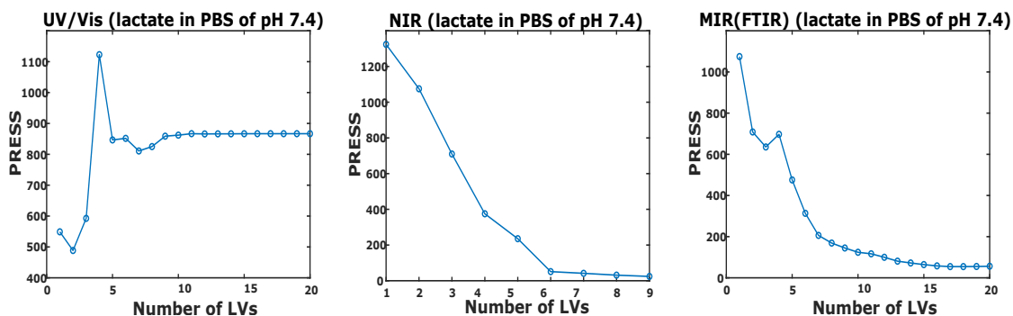
Figure 5.8: Prediction Error Sum of Squares (PRESS) versus number of latent variables (LV). (a) The number of LVs in the UV/Vis spectral region used was 2; (b) The number of LVs in the NIR spectral region used was 8; (c) The number of LVs in the MIR spectral region used was 18.
