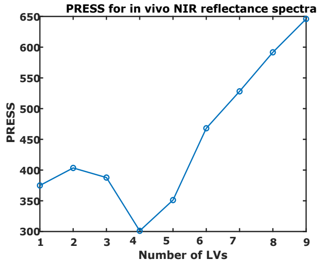
Figure 9.5: Prediction Error Sum of Squares (PRESS) versus number of latent variables (LV) for in-vivo NIR reflectance spectra. The number of LVs used was 4.
