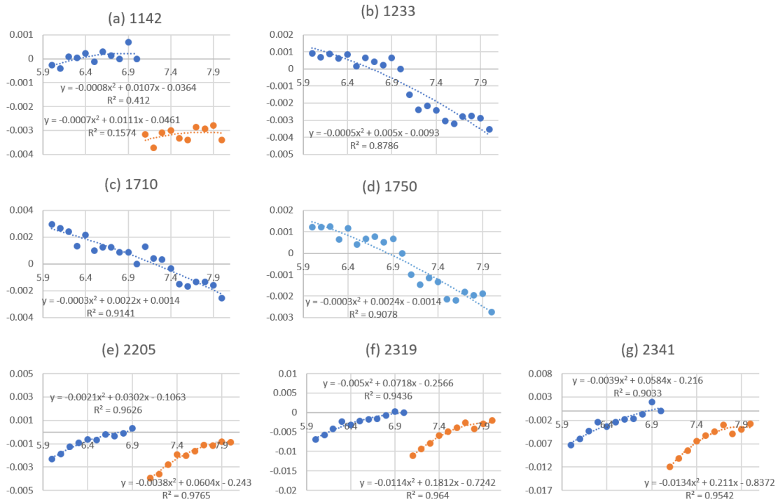
Figure 6.3: Absorbance vs pH of wavelengths: (a) 1142nm (b) 1233nm (c) 1710nm (d) 1750nm (e) 2205nm (f) 2319nm (g) 2341nm. Figure taken from 254 .
