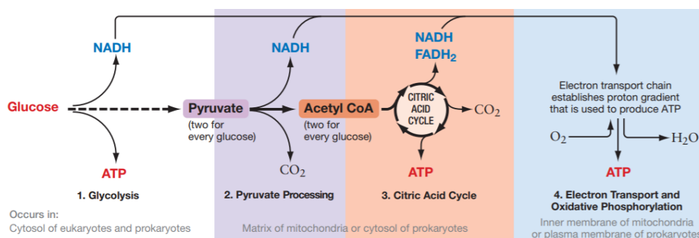
Figure 2.3: Aerobic Respiration is a metabolic pathway of converting glucose to high energy molecules (or ATP). There are four processes and they occur in the cellular level. The first three processes, i.e., 1. Glycolysis 2. Pyruvate Processing and 3. Citric Acid Cycle, produce NADH and/or Flavin Adenine Dinucleotide FADH_2 by oxidizing glucose. These electron carriers (NADH or FADH_2 ) are then fed into the electron transport chain for oxidative phosphorylation. Image taken from 45 .
