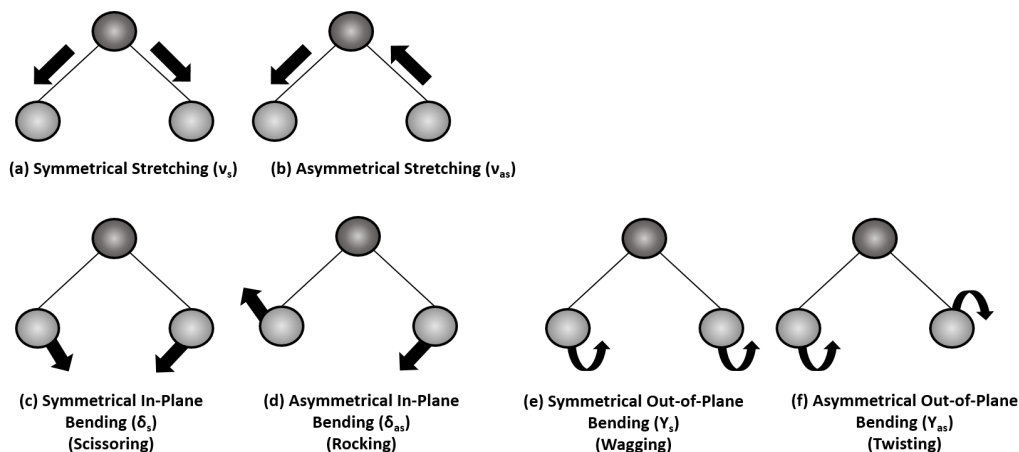
Figure 3.4: Fundamental modes of vibrations in a molecule (a) Symmetrical Stretching ( \nu_s ), (b) Asymmetrical Stretching ( \nu_{as} ), (c) Symmetrical In-Plane Bending ( \delta_s ) (Scissoring), (d) Asymmetrical In-Plane Bending ( \delta_{as} ) (Rocking), (e) Symmetrical Out-of-Plane Bending ( \gamma_s ) (Wagging) and (f) Asymmetrical Out-of-Plane Bending ( \gamma_{as} ) (Twisting) (Redrawn from: 138 ).
