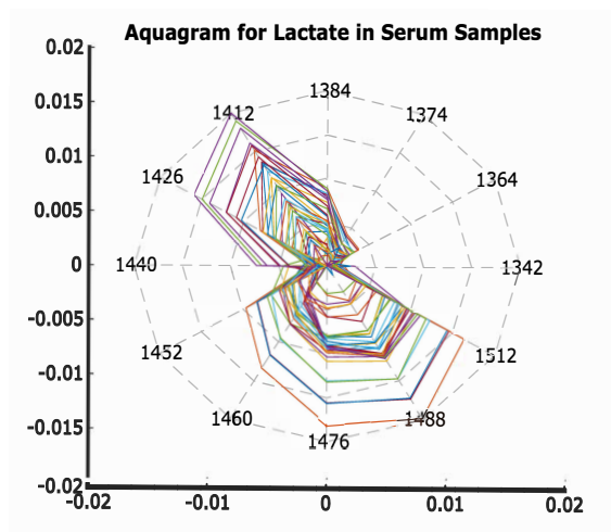
Figure 7.1: Aquagram for lactate in Serum samples in Water Absorbance Bands (WAB): 1300-1600 nm , showing Water Absorbance Spectral Pattern (WAPS) in the Water matrix co-ordinates (WAMACS) of varying concentrations of lactate in human serum samples. The WAMACS: 1342, 1364, 1374, 1384, 1412, 1426, 1440, 1452, 1460, 1476, 1488 and 1512 depicts molecular conformations which arises due to water-NIR light-lactate molecule interactions.
