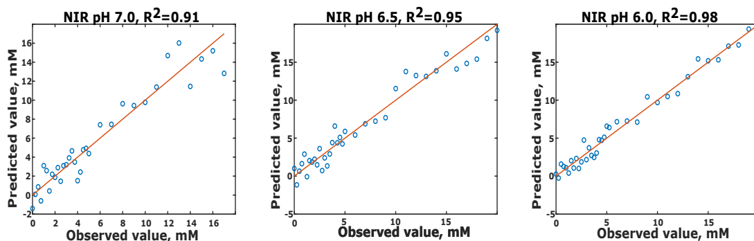
Figure 6.8: Observed (known) lactate concentration versus the Predicted concentrations of thirty-seven PBS samples of lactate prepared using solution stoichiometry. The correlation coefficient ( R^2 ) and the root mean squared error of cross validation (RMSECV) for each set are also shown. (a) The Coefficient of Determination ( R^2 ) and the root mean squared error of cross validation (RMSECV) for NIR pH 7 set is 0.91 and 0.63 mM , respectively; (b) The Coefficient of Determination ( R^2 ) and the root mean squared error of cross validation (RMSECV) for NIR pH 6.5 set is 0.95 and 0.44 mM , respectively; (c) The Coefficient of Determination ( R^2 ) and the root mean squared error of cross validation (RMSECV) for NIR pH 6 set is 0.98 and 0.42 mM , respectively.
