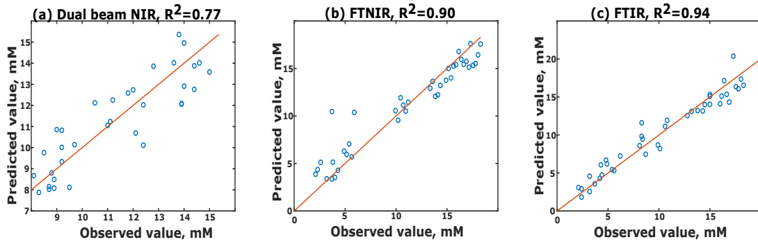
Figure 7.3: Observed (known) lactate concentration versus the Predicted concentrations of forty-one samples of lactate in Human Serum. The correlation coefficient ( R^2 ) and the Root Mean Squared Error of Cross Validation (RMSECV) for each set are also shown. (a) The Coefficient of Determination ( R^2 ) and the Root Mean Squared Error of Cross Validation (RMSECV) for dual beam dispersive NIR data-set are 0.77 and 1.11 mM respectively; (b) The Coefficient of Determination ( R^2 ) and the Root Mean Squared Error of Cross Validation (RMSECV) for FTNIR set are 0.90 and 1.75 mM respectively; (c) The Coefficient of Determination ( R^2 ) and the Root Mean Squared Error of Cross Validation (RMSECV) for MIR (FTIR) set are 0.94 and 1.31 mM respectively.
