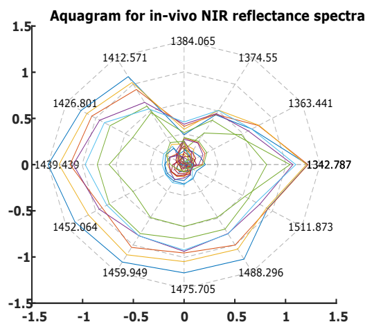
Figure 9.4: Aquagram for in-vivo NIR reflectance spectra from upper part of thumb obtained by NIRQuest portable spectrometer from Ocean Optics ( Largo, FL, USA ). Water Absorbance Bands (WAB): 1300-1600nm, showing Water Absorbance Spectral Pattern (WAPS) in the Water matrix co-ordinates (WAMACS) of varying concentrations of lactate in-vivo . The WAMACS: 1342.787, 1363.441, 1374.55, 1384.065, 1412.571, 1426.801, 1439.439, 1452.064, 1459.949, 1475.705, 1488.296 and 1511.873 depicts molecular conformations which arises due to water-NIR light-lactate molecule interactions.
