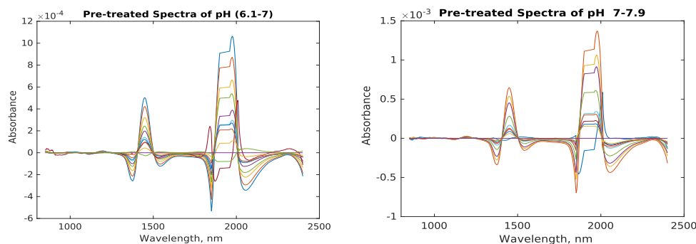
Figure 6.2: Pre-treated Spectra, Extended Multiplicative Scatter Correction (EMSC) and Savitzky-Golay filtering of pH 6-8. (a) Pre-treated Spectra of pH 6.1-7 (b) Pre-treated Spectra of pH 7-7.9. Figure taken from 254 .
