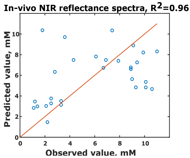
Figure 9.6: Observed (known) lactate concentration versus the Predicted concentrations for in-vivo NIR reflectance spectra. The correlation coefficient ( R^2 ) and the Root Mean Squared Error of Cross Validation (RMSECV) are 0.96 and 3.22 mM , respectively.
