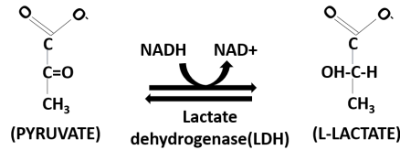
Figure 2.4: Under anaerobic conditions, instead of entering the Kerb's cycle or Citric Acid Cycle, pyruvate and NADH, which are produced during glycolysis, are reduced to lactate and NAD + . This reaction is catalysed by the tetrameric enzyme Lactate dehydrogenase (LDH). Picture re-drawn from 46 .
