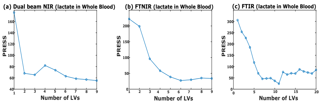
Figure 8.2: Prediction Error Sum of Squares (PRESS) versus number of latent variables (LV) for 41 samples of Lactate solutions in whole blood for dual beam dispersive NIR data-set, FTNIR data-set and MIR (FTIR) data-set. (a) The number of LVs for the dual beam dispersive NIR data-set used was 9; (b) The number of LVs for the FTNIR data-set used was 6; (c) The number of LVs for the MIR data-set used was 11.
