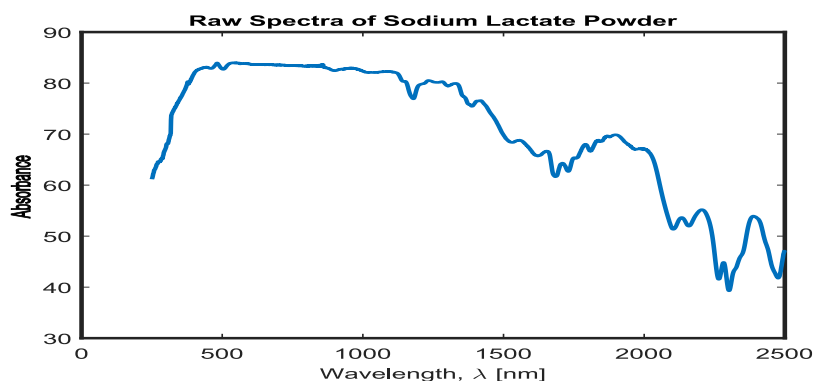
Figure 5.1: Raw spectrum of Sodium L-Lactate Powder through Reflectance Spectroscopy in 250-2500 nm .
