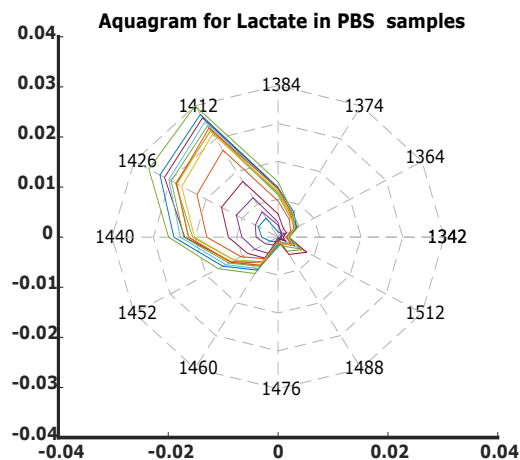
Figure 5.7: Aquagrams for lactate in PBS samples in Water Absorbance Bands (WAB): 1300-1600 nm , showing Water Absorbance Spectral Pattern (WAPS) in the Water matrix co-ordinates (WAMACS) of varying concentrations of lactate in PBS samples. The WAMACS: 1342, 1364, 1374, 1384, 1412, 1426, 1440, 1452, 1460, 1476, 1488 and 1512 depicts molecular conformations which arises due to water-NIR light-lactate molecule interactions.
