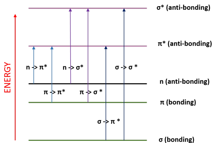
Figure 3.2: The allowed electronic transitions in energy band diagram are: n - \pi^* , \pi - \pi^* , n - \sigma^* , \pi - \sigma^* , \sigma - \pi^* , \sigma - \sigma^* (Redrawn from: 134 ).
