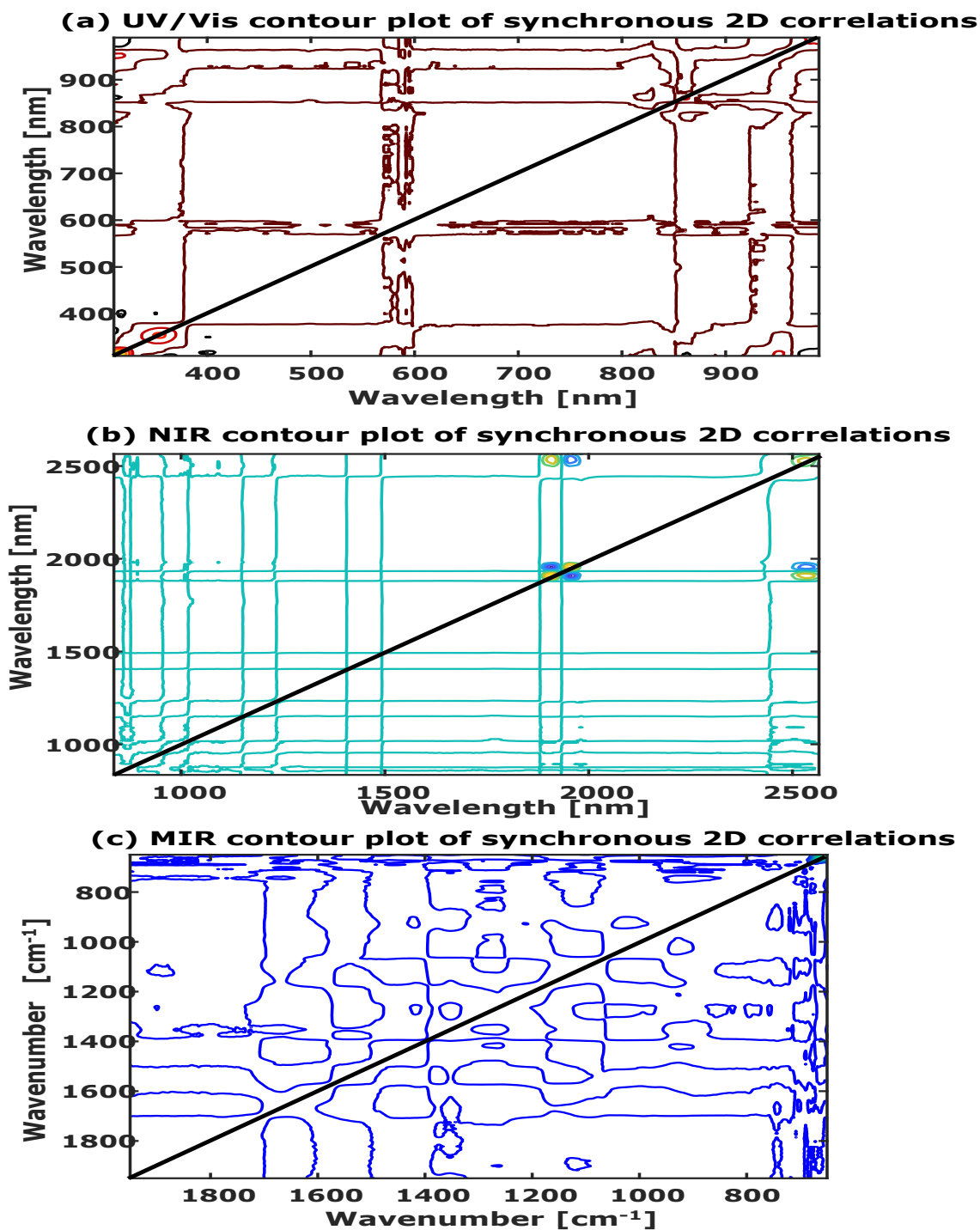
Figure 5.4: Two-dimensional synchronous correlation plot depicting the correlation changes in the 36 spectra in the UV/Vis, NIR and MIR (FTIR) Spectra. (a) 2D synchronous correlation plot in the UV/Vis spectral region; (b) 2D synchronous correlation plot in the NIR spectral region; (c) 2D synchronous correlation plot in the MIR spectral region.
