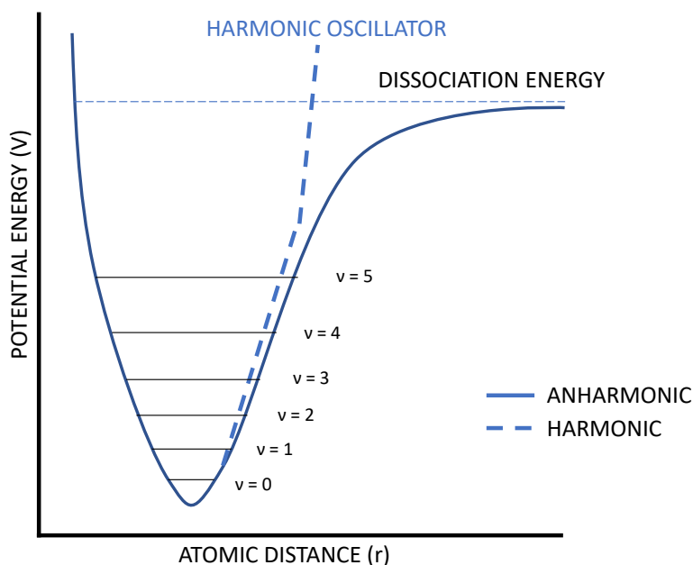
Figure 3.5: Model of the harmonic and anharmonic oscillators with vibrational energy levels (Redrawn from: 139 ).
