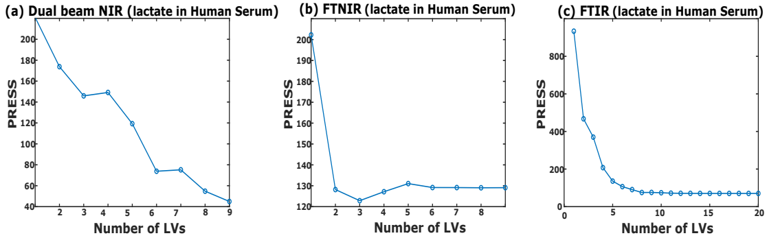
Figure 7.2: Prediction Error Sum of Squares (PRESS) versus number of latent variables (LV) for of 41 samples of Lactate solutions in Human Serum for dual beam dispersive NIR data-set, FTNIR data-set and MIR (FTIR) data-set. (a) The number of LVs for the dual beam dispersive NIR data-set used was 9; (b) The number of LVs for the FTNIR data-set used was 3; (c) The number of LVs for the MIR data-set used was 18.
