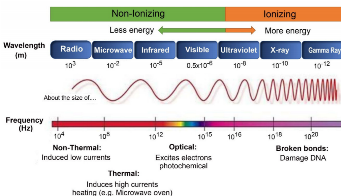
Figure 4.5: The Electromagnetic Spectrum (schematic representation) from the Radio (Wavelength: 10^3m , Frequency: 10^4 Hz) to the Gamma Rays (Wavelength: 10^{-12}m , Frequency: 10^{20} Hz). The Microwave, Infrared and Visible are Non-Ionizing waves, whereas, the Ultraviolet has more energy and can ionize a molecule. Picture taken from 210 .
