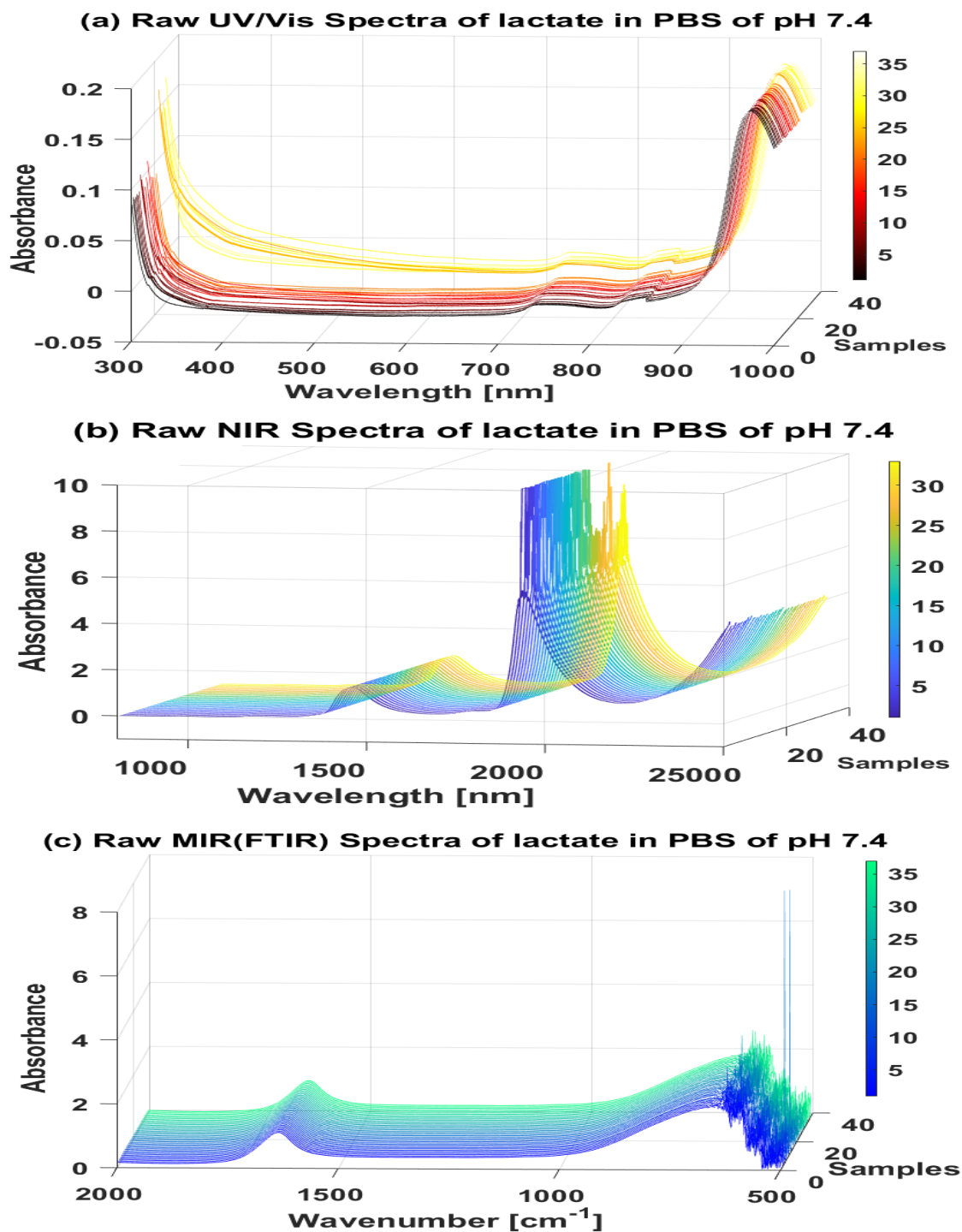
Figure 5.2: Raw spectra of thirty-seven Sodium (Na)-L-Lactate solutions of varying concentration ranging between 0–20 mM in Phosphate Buffer Saline (PBS) samples. (a) UV/Vis (300–1000 nm ) raw spectra of 37 samples of Na-L-Lactate (0–20 mM ) in PBS; (b) NIR (800–2600 nm ) raw spectra of 37 samples of Na-L-Lactate (0–20 mM ) in PBS; (c) MIR (2000–500 cm -1 ) raw spectra of 37 samples of Na-L-Lactate (0–20 mM ) in PBS.
