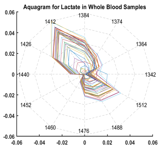
Figure 8.1: Aquagram for lactate in Whole Blood samples in Water Absorbance Bands (WAB): 1300-1600nm, showing Water Absorbance Spectral Pattern (WAPS) in the Water matrix co-ordinates (WAMACS) of varying concentrations of lactate in whole blood samples. The WAMACS: 1342, 1364, 1374, 1384, 1412, 1426, 1440, 1452, 1460, 1476, 1488 and 1512 depicts molecular conformations which arises due to water-NIR light-lactate molecule interactions.
