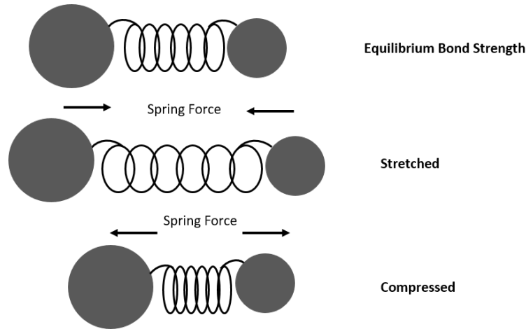
Figure 3.3: Mechanical Model of a diatomic system, where there are two masses, M and m , connected by a spring (Redrawn from: 137 ).
