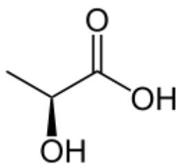
Figure 2.1: Lactic Acid (Chemical Formula).
