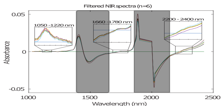
Figure 5.5: The regions of interest in the NIR spectral region pertinent to high lactate concentration changes are 1050-1220 nm , 1660-1780 nm and 2200-2400 nm . The grey areas 1450-1600 nm and 1960-2250 nm are influenced by OH bonds. Figure taken from 250 .
