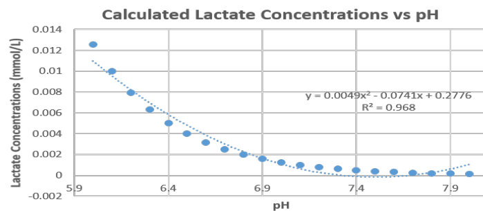
Figure 6.1: Theoretically calculated concentrations of lactate vs pH (6-8) using the Henderson- Has-selbach equation. The fit of the curve follows the equation of y = 0.0049x^2 - 0.0741x + 0.2776 , with R^2=0.968 . Figure taken from 254 .
