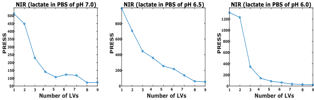
Figure 6.5: Prediction Error Sum of Squares (PRESS) versus number of latent variables (LV). (a) The number of LVs in the NIR spectral region for pH 7 used was 8; (b) The number of LVs in the NIR spectral region for pH 6.5 used was 8; (c) The number of LVs in the NIR spectral region for pH 6 used was 8.
