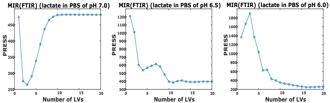
Figure 6.6: Prediction Error Sum of Squares (PRESS) versus number of latent variables (LV). (a) The number of LVs in the MIR spectral region for pH 7 used was 3; (b) The number of LVs in the MIR spectral region for pH 6.5 used was 12; (c) The number of LVs in the MIR spectral region for pH 6 used was 16.
