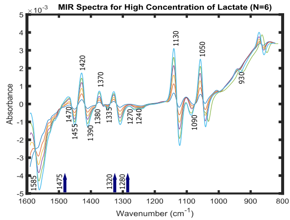
Figure 5.6: Wavenumbers of interest in the MIR spectral region 800\text{--}1600\text{ cm}^{-1} , pertinent to high lactate concentration changes. The set of six spectra (after pre-processing) of very high concentration of lactate in PBS (100 (dark green), 200 (orange), 300 (yellow), 400 (red), 500 (light green) and 600 mM (blue)) obtained in the MIR(FTIR) range. The wavenumbers 860\text{ cm}^{-1} , 930\text{ cm}^{-1} , 1050\text{ cm}^{-1} , 1090\text{ cm}^{-1} , 1130\text{ cm}^{-1} , 1240\text{ cm}^{-1} , 1270\text{ cm}^{-1} , 1280\text{ cm}^{-1} , 1320\text{ cm}^{-1} , 1335\text{ cm}^{-1} , 1370\text{ cm}^{-1} , 1380\text{ cm}^{-1} , 1390\text{ cm}^{-1} , 1420\text{ cm}^{-1} , 1470\text{ cm}^{-1} , 1475\text{ cm}^{-1} and 1585\text{ cm}^{-1} could be visibly seen in the spectra. Figure taken from 251 .
