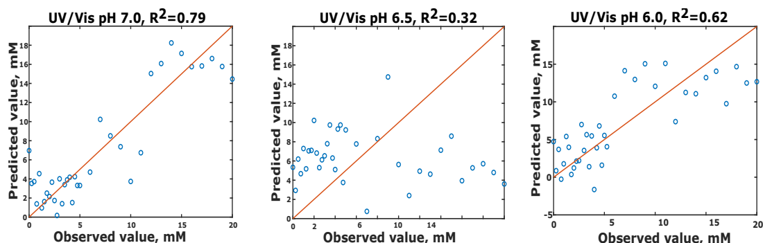
Figure 6.7: Observed (known) lactate concentration versus the Predicted concentrations of thirty-seven PBS samples of lactate prepared using solution stoichiometry. The correlation coefficient ( R^2 ) and the root mean squared error of cross validation (RMSECV) for each set are also shown. (a) The Coefficient of Determination ( R^2 ) and the root mean squared error of cross validation (RMSECV) for UV/Vis pH 7 set is 0.79 and 2.73 mM , respectively; (b) The Coefficient of Determination ( R^2 ) and the root mean squared error of cross validation (RMSECV) for UV/Vis pH 6.5 set is 0.32 and 6.27 mM , respectively; (c) The Coefficient of Determination ( R^2 ) and the root mean squared error of cross validation (RMSECV) for UV/Vis pH 6 set is 0.62 and 4.17 mM , respectively.
