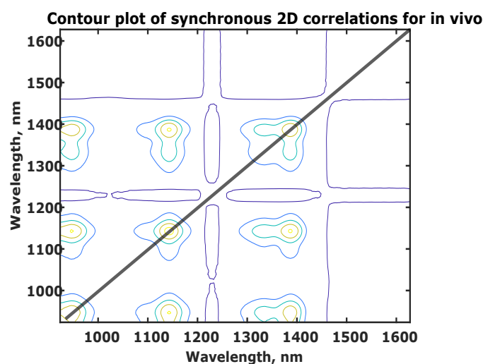
Figure 9.3: Synchronous 2D correlations contour plot for in-vivo NIR reflectance spectra obtained from upper part of thumb obtained by NIRQuest portable spectrometer from Ocean Optics ( Largo, FL, USA ).
