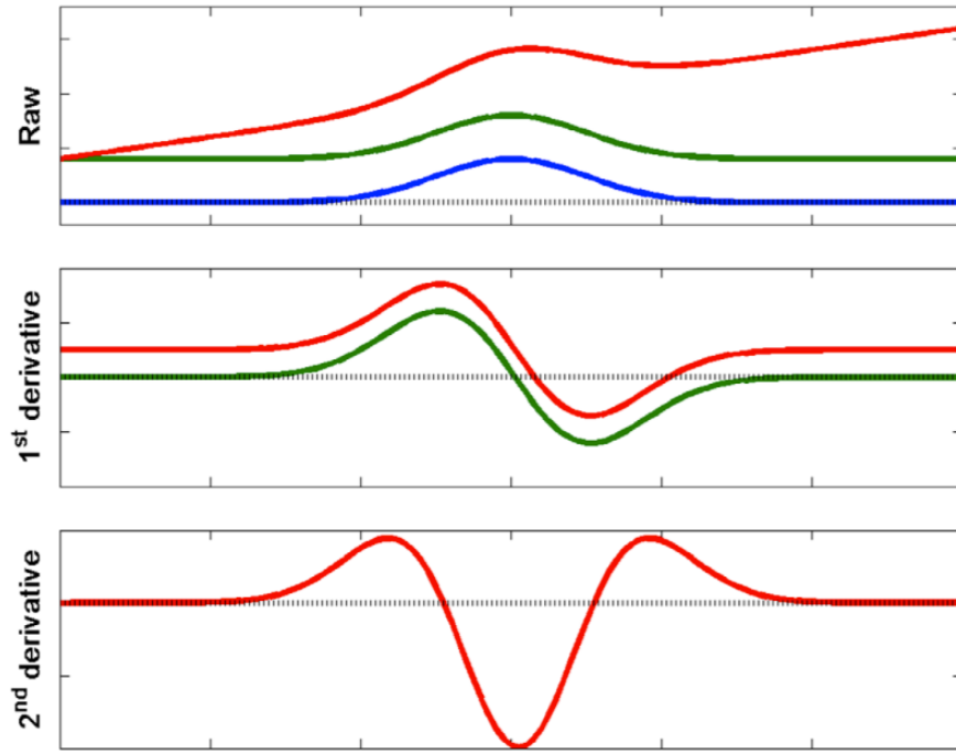
Figure 3.10: The 1 st and 2 nd derivative of the raw spectrum. Picture taken from 157 .
