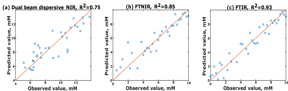
Figure 8.3: Observed (known) lactate concentration versus the Predicted concentrations of forty-one samples of lactate in whole blood. The correlation coefficient ( R^2 ) and the Root Mean Squared Error of Cross Validation (RMSECV) for each set are also shown. (a) The Coefficient of Determination ( R^2 ) and the Root Mean Squared Error of Cross Validation (RMSECV) for dual beam dispersive NIR data-set are 0.75 and 1.23 mM respectively; (b) The Coefficient of Determination ( R^2 ) and the Root Mean Squared Error of Cross Validation (RMSECV) for FTNIR set are 0.85 and 1.02 mM respectively; (c) The Coefficient of Determination ( R^2 ) and the Root Mean Squared Error of Cross Validation (RMSECV) for MIR (FTIR) set are 0.93 and 0.78 mM respectively.
