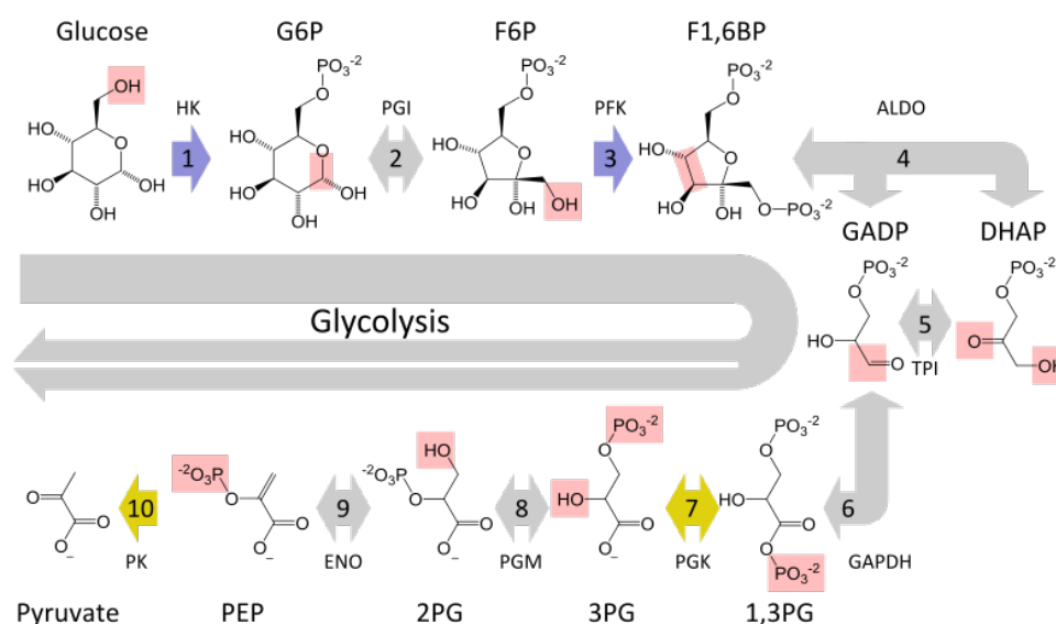
Figure 2.2: The 10 step Gustav Emben, Otto Meyerhof, Jakub Karol Parnas (EMP) or the ‘ glycolytic pathway ’ which converts glucose to pyruvate. The red boxes indicate chemical modifications in the intermediate metabolites by different enzymes. Adenosine Tri Phosphate (ATP) is consumed in the first three steps (shown in blue) and produced in the next seven steps (shown in yellow). Steps 6-10 are repeated twice per glucose molecule and hence, there is a net increase (or production) of ATP in the process. HK= Hexokinase, G6P= Glucose 6-phosphate, PGI= Glucose-6-phosphate isomerase, F6P= Fructose 6-phosphate, PFK= Phosphofructokinase-1, F1,6BP= Fructose 1,6-bisphosphate, ALDO= Fructose-bisphosphate aldolase, DHAP= Dihydroxyacetone phosphate, GADP= Glyceraldehyde 3-phosphate, TPI= Triosephosphate isomerase, GAPDH= Glyceraldehyde-3-phosphate dehydrogenase, 1,3PG= 1,3-Bisphosphoglycerate, PGK= Phosphoglycerate kinase, 3PG= 3-Phosphoglycerate, PGM= Phosphoglycerate mutase, 2PG= 2-Phosphoglycerate, ENO= Phosphopyruvate hydratase (enolase), PEP= Phosphoenolpyruvate, PK= Pyruvate kinase. Picture taken from 43 .
