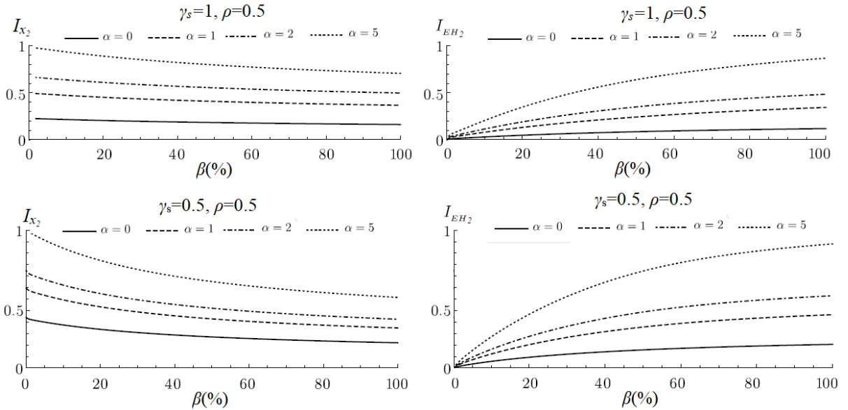
Figure 8. Motion control and energy harvesting performance indices in Eq. (33) normalized to their peak value for correlated ( \rho=0.5 ) white noise force-excited EH-TMDI-equipped 2-DOF primary structures with \zeta_{s,1} = \zeta_{s,2} = 5\% , \zeta_{EH} = 10\% , \zeta_p = 1\% , \mu_I = 1\% , and \mu_s = 1 , plotted against the inertance ratio \beta .
