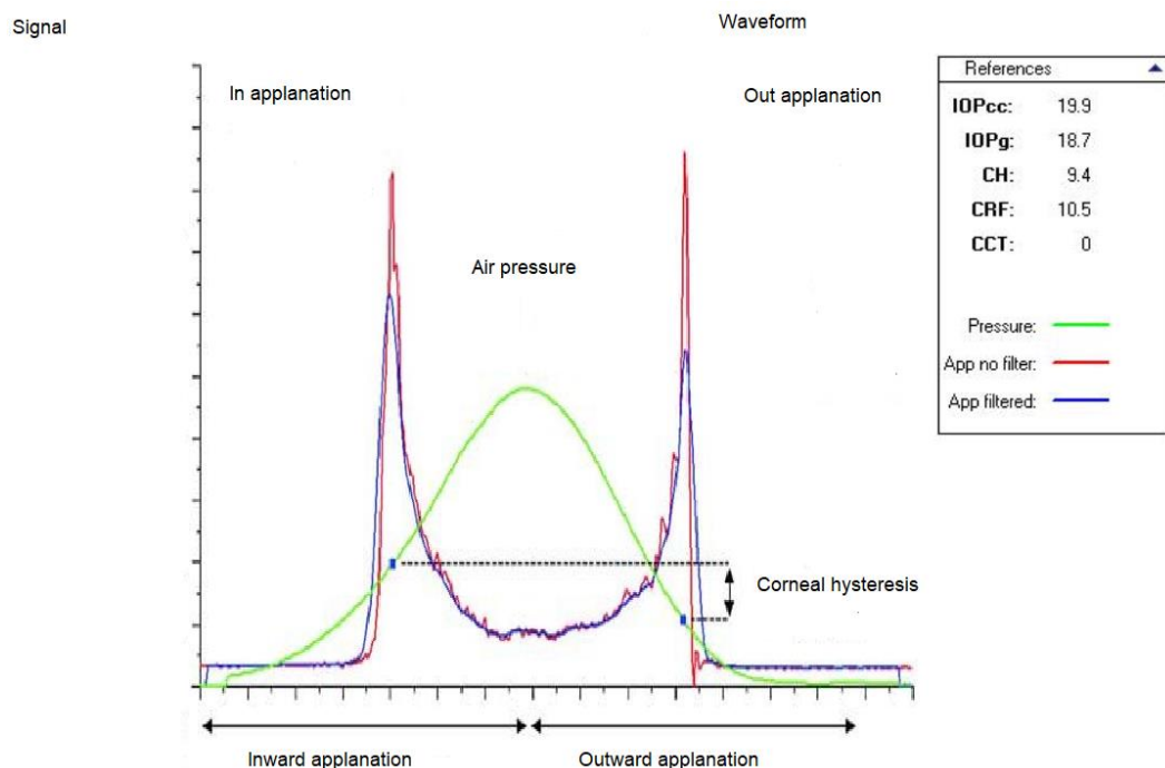
Figure 4.5. Ocular Response Analyser (ORA) graphical plot comprising 3 curves: pressure of air applied to the cornea (green), raw signal of applanation detection system (red), and a filtered version of the latter to identify optimum points of applanation (blue)
