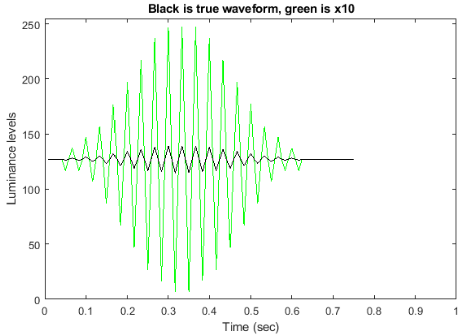
Figure 3.2. – Flicker modulation stimulus within cosine envelope
