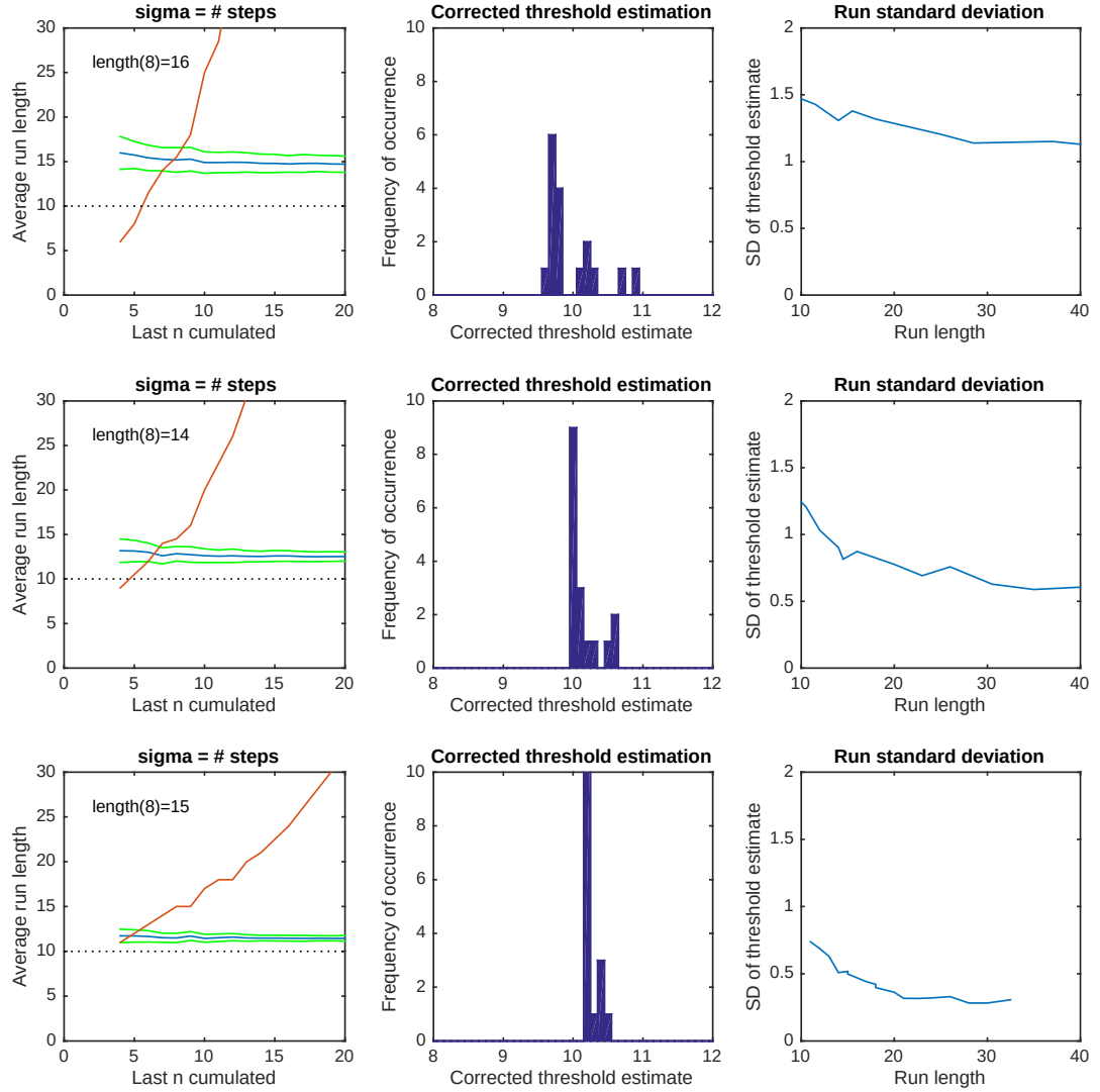
Figure 3.4. Simulation of the performance of the Accelerator staircase method at three levels of step size relative to the noise sigma controlling threshold level (0.5, 1 and 2 decilogs top to bottom row respectively). Column 1: Overlays of average run length (red curves) and threshold estimate (blue curves) \pm 1 standard error of the mean (SEM) (green curves) as a function of the criterion cumulation length for the last n values for the sigma estimate. Dashed line is the simulated threshold level. Inset gives the average run length for a criterion cumulation length of 8 steps. Column 2: Histograms of the corrected threshold estimates on each trial simulation. Column 3: Standard deviation (SD) of the threshold estimates as a function of run length. Simulation provided by Christopher Tyler.
