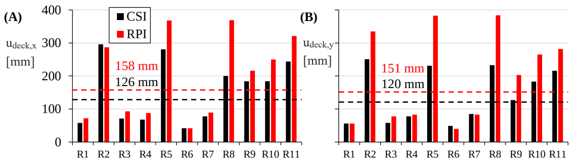
Fig. 6-19 Peak superstructure relative displacements of segment (P1-P2) in the (A) longitudinal ( u_{deck,x} ) and (B) transverse directions ( u_{deck,y} ) for the CSI and RPI bridges with tall piers. Results obtained when subject to the scaled Ri.
