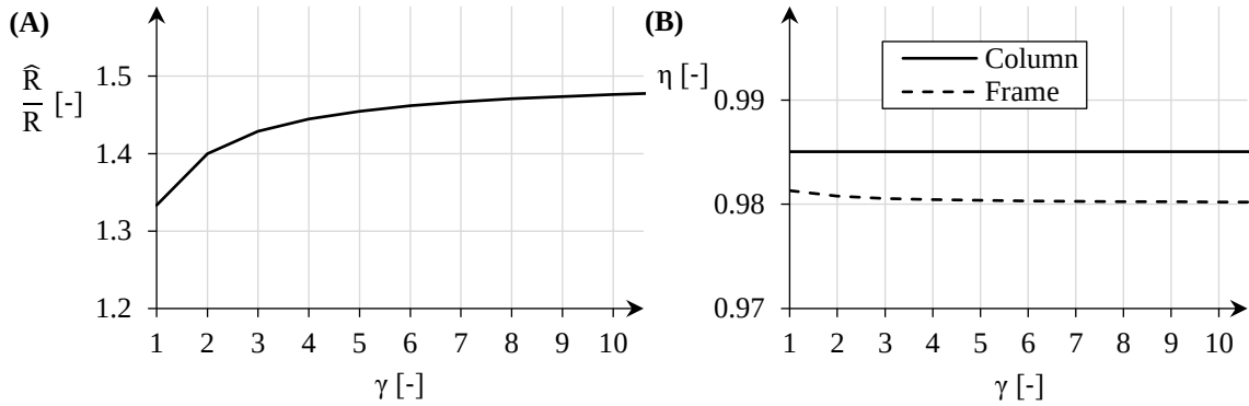
Fig. 2-15 (A) Ratio \hat{R}/R as described by Eq. (2-18) and (B) CoR at the rocking interfaces ( \eta ) for free-standing rocking columns (Housner 1963) and for relevant symmetric frames (Makris & Vassiliou 2013), accounting for the influence of the superstructure mass effect ( \gamma ). Results obtained when \alpha = 0.1 rad.
