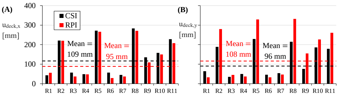
Fig. 6-8 Peak superstructure relative displacements of segment (P1-P2) in the (A) longitudinal ( u_{deck,x} ) and (B) transverse directions ( u_{deck,y} ) for the CSI and RPI bridges with short piers. Results obtained when subject to the scaled Ri.
