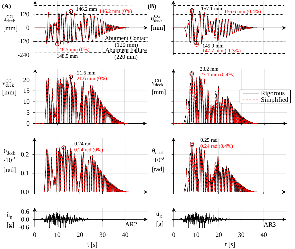
Fig. 4-12 Histories of the longitudinal ( u_{deck}^{CG} ) and vertical displacements ( v_{deck}^{CG} ) as well as superstructure rotation ( \theta_{deck} ) for the highly asymmetric bridge with rocking piers of \bar{h} = 2 , considering the rigorous and simplified models for \partial\phi_{CD}/\partial\phi , \partial^2\phi_{CD}/\partial\phi^2 , \partial\theta_{deck}/\partial\phi and \partial^2\theta_{deck}/\partial\phi^2 . Results obtained when subject to (A) AR2 and (B) AR3.
