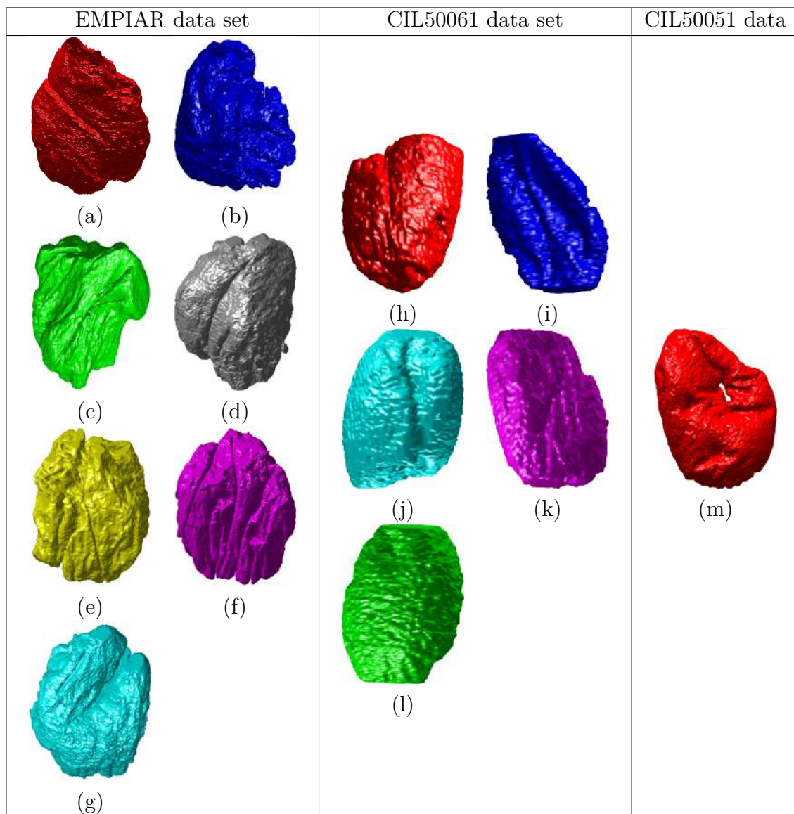
Fig. 5.10 Final results of the automated segmentation of thirteen Nuclear Envelopes (NEs) displayed as rendered volumetric surfaces for Wild type and Chlamydia trachomatis-infected HeLa cells. Surface rendering of thirteen Nuclear Envelopes (NEs), different colours are used for visualisation purposes. Seven Wild-type HeLa cells (EMPIAR data set - left column) and six Chlamydia trachomatis-infected HeLa cells from two data sets (centre and right column). (a-g) Wild-type HeLa cells. In each cell, notice the notches that travel up-down along the nuclei (grey (d), yellow (e), purple (f), and cyan (g) cell) and invaginations. Voxel size of Wild-type HeLa cells is 10 \times 10 \times 50 nm. (h-l) Segmented cells from CIL50061 data set. Cells in this data set are 12 hours post infection (hpi) and voxel size 8.6 \times 8.6 \times 60 nm. (m) A cell from CIL50051 with 28 hpi and voxel size is 3.6 \times 3.6 \times 60 nm. Notice the hole of this particular cell.
