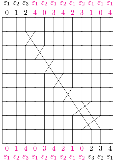
FIGURE 16. We let h = 3 , \ell = 1 , e = 5 and \alpha = \varepsilon_3 - \varepsilon_1 . The adjustment term \text{adj}_{\emptyset\alpha}^{\alpha\emptyset} is illustrated.
