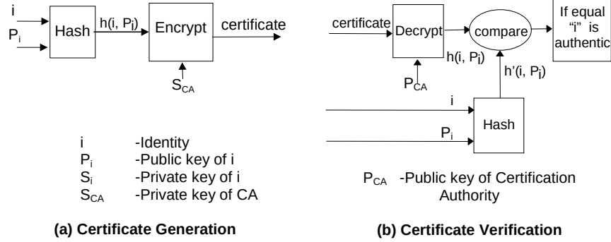
Figure 1 Certificate Generation and Verification Process
