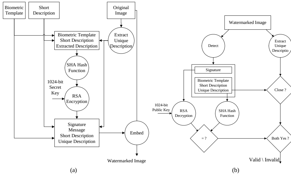
Fig. 1. Cryptographic Encoder / Decoder
