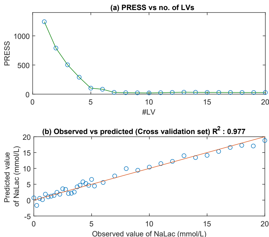
Figure 5. (a) The graph of PRESS versus number of latent variables (LV) for NIR spectra. Optimal number of LVs used for building the PLS model were eight, and (b) predicted NaLac concentration vs. the reference NaLac concentration of thirty-seven PBS samples. The correlation coefficient ( R^2 ) and root mean square error of cross-validation (RMSECV) were 0.977 and 0.89 mmol/L, respectively.
