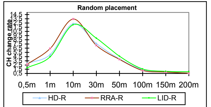
Fig. 6 Comparison of cluster head change rate: 200Nodes, 5km/h.
