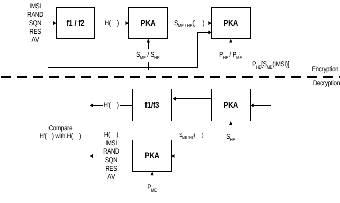
Fig. 5. Encryption/Decryption in AAKA using Public Key Cryptography and Digital Signatures
