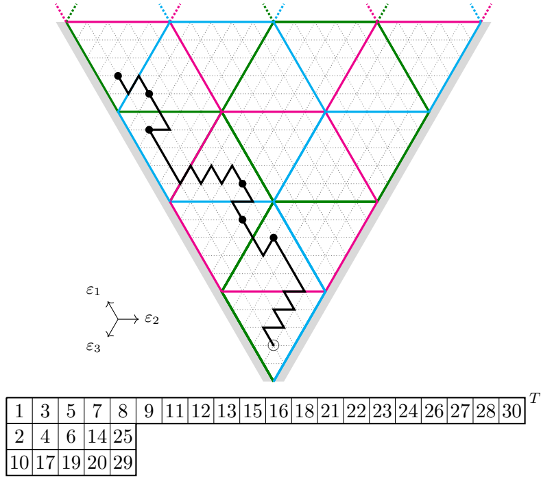
FIGURE 1. An alcove path in \mathbb{E}_{3,1}^+ in \text{Path}_{h,\ell}(3^5, 1^{15}) and the corresponding tableau in \text{Std}(3^5, 1^{15}) . The black vertices denote vertices on the path in the orbit of the origin.
