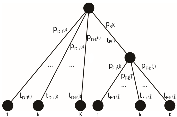
Figure 3. The K -Class Standard Tree for Ordered Processes
