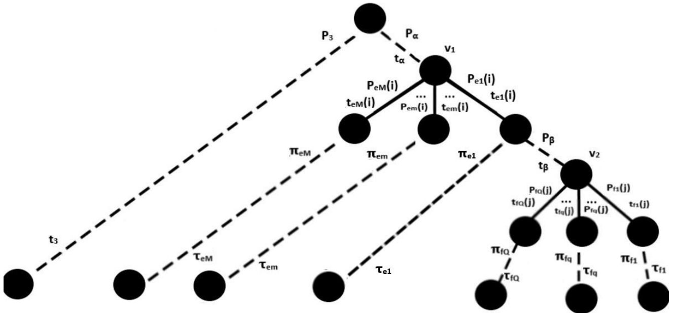
Figure 5. Paths from the source of an arbitrary MPT to a terminal vertex. A factor with levels indexed by i selectively influences one vertex and a factor with levels indexed by j selectively influences a following vertex. All possible paths to a vertex of one particular response class are illustrated.
