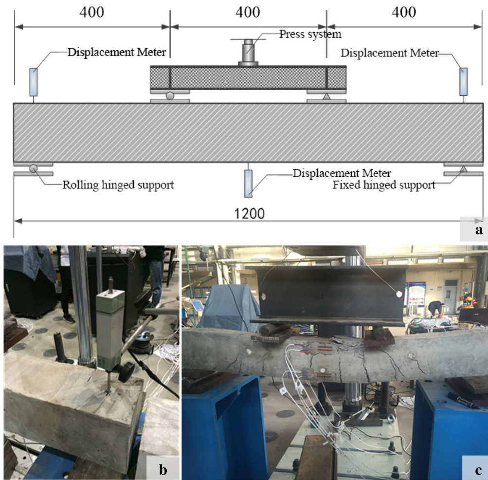
Fig. 7 Loading procedure
