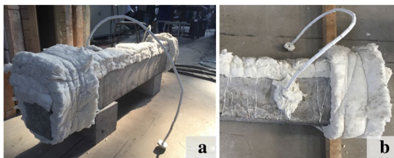
Fig. 3 Three-sided fire exposure and thermocouple layout
