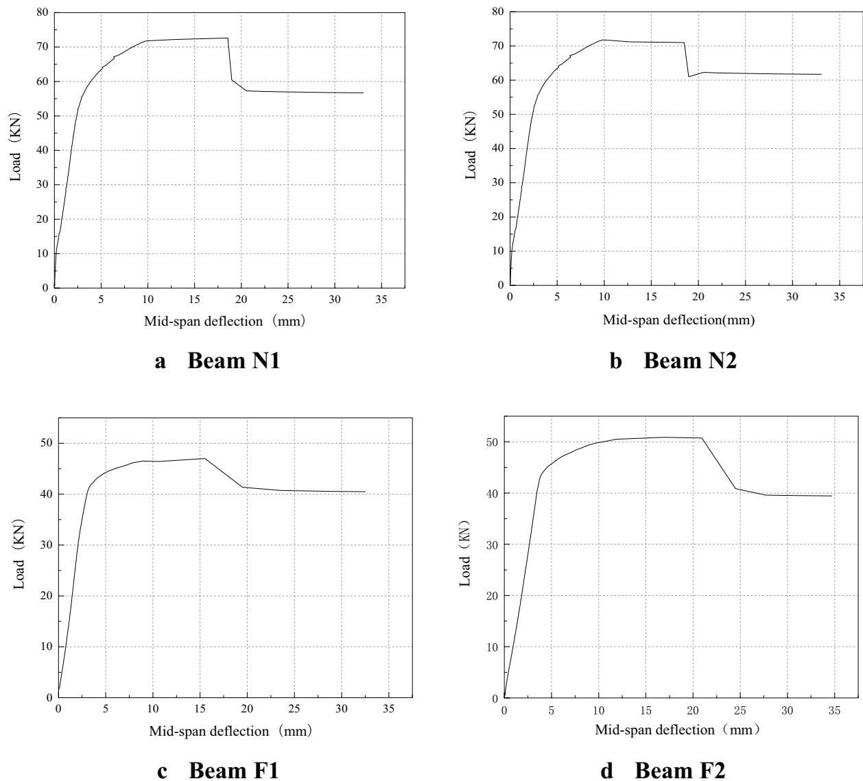
Fig. 8 Load-deflection curves of different beams
