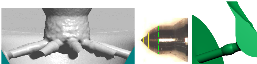
Figure 3.29: Cavitation erosion effect on the geometry: experimental visualization extracted from [92] (left and center) and deformed geometrical model (right).
