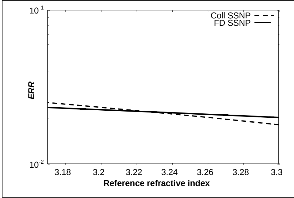
Figure 8 Error in propagation with the reference refractive index for the benchmark step-index waveguide (SIW1) for propagation up to 100 \mu\text{m} with step size 0.1 \mu\text{m} at 40°.
