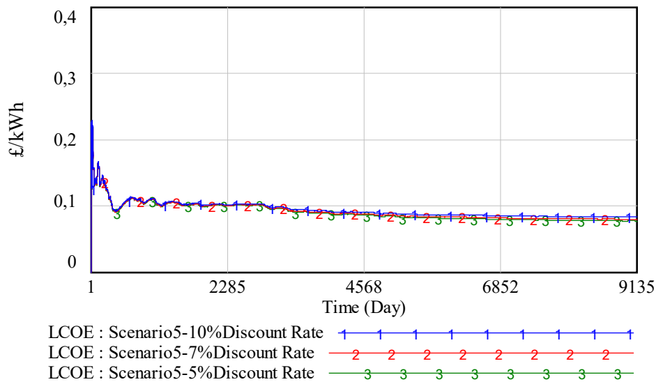
Figure 6-11: LCOE for Different Discount Rate
