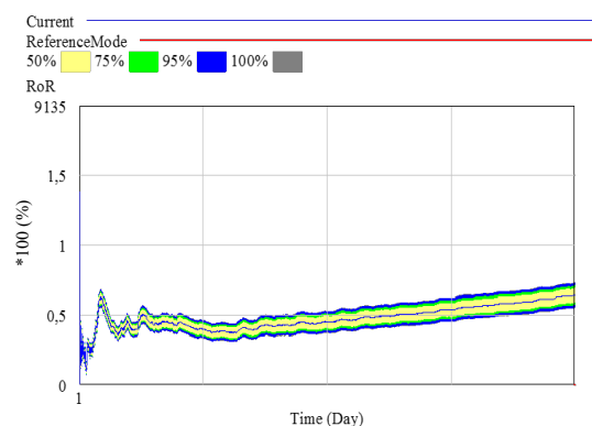
Figure 6-18: ROR vs Price of Exporting Electricity to the grid
