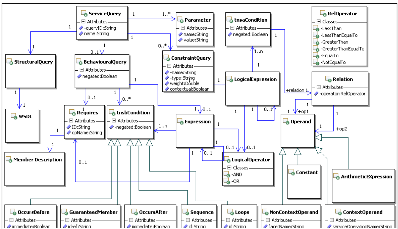
Fig 2: UML representation of SerDiQueL
