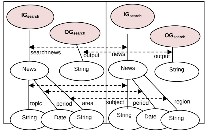
Fig 7: Example of data type graphs
