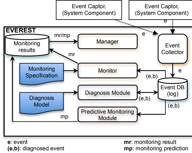
Figure 2. EVEREST architecture
