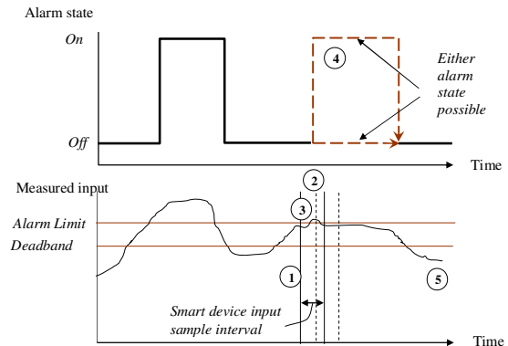
Figure 4. Non-determinism due to sample rate
