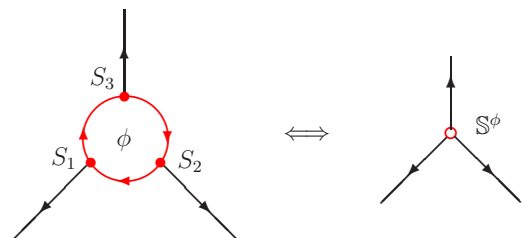
FIG. 1: (Color online) Ring junction with local S -matrices \{S_j : j = 1, 2, 3\} and magnetic flux \phi (left) and its Y-junction counterpart with equivalent total scattering matrix \mathbb{S}^\phi (right).
