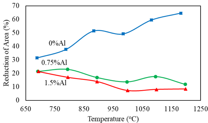
Figure 2-27 The hot ductility of TWIP steel at different Al content for the base composition: 0.6%C, 0.008%S, 18%Mn and 0.01%N [101].
