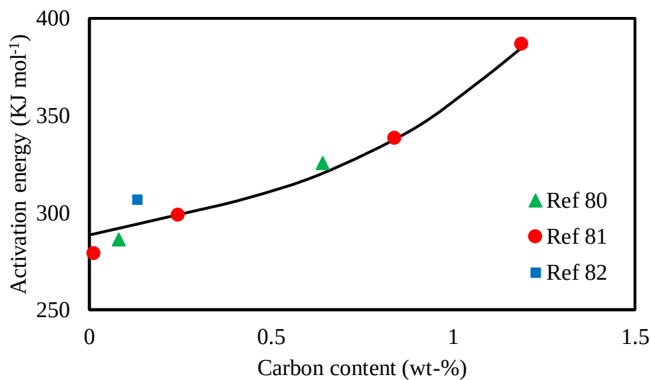
Figure 2-21 Influence of carbon content on activation energy [80-82].
