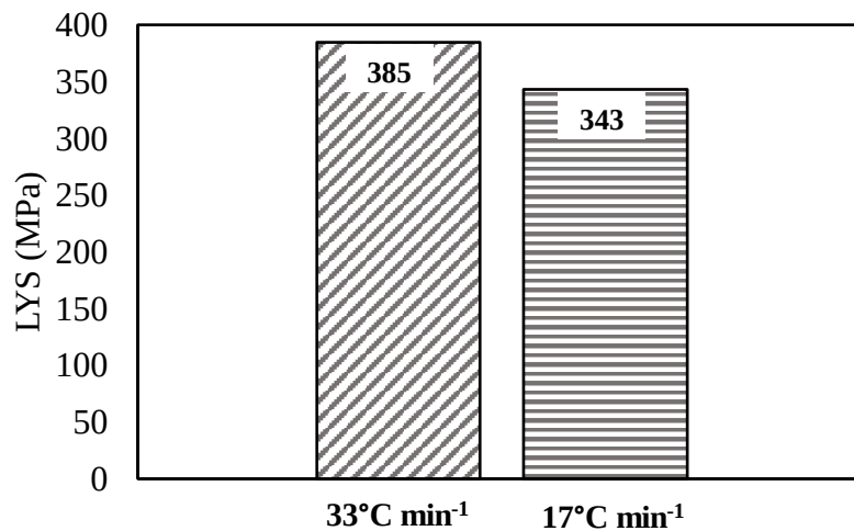
Figure 5-10 LYS of the 0.018%Nb steel at both cooling rates ( 33 and 17^{\circ}\text{C min}^{-1} ).
