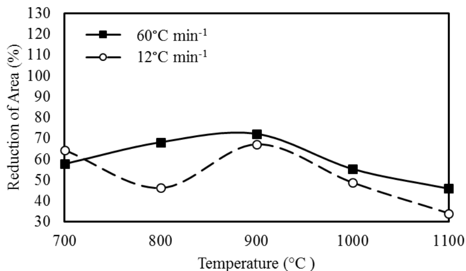
Figure 4-5 The hot ductility of TWIP steel with low Ti/N ratio at 12 and 60°C min -1 .
