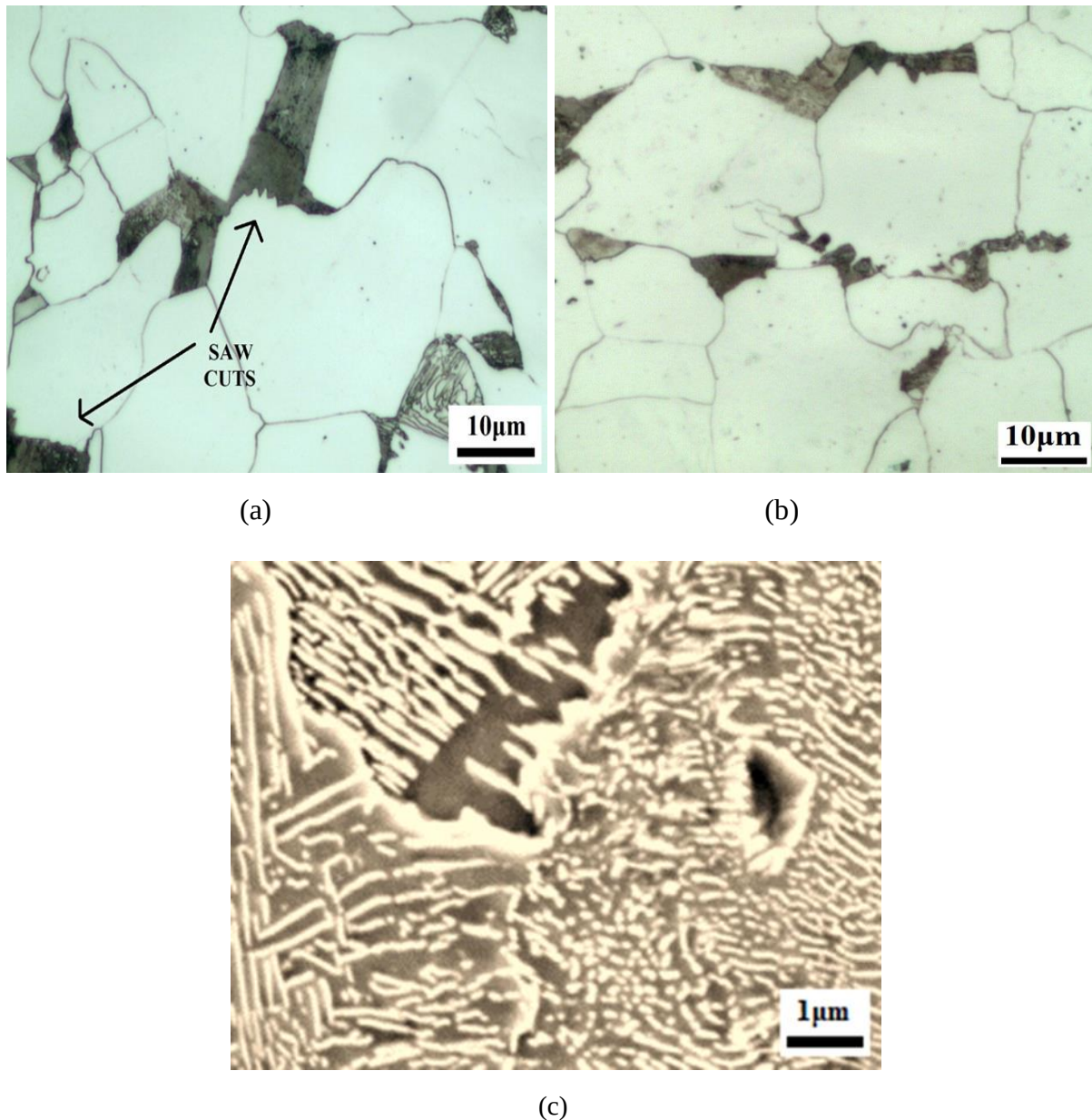
Figure 5-22 (a) OM photo showing teeth or saw cuts in the hot rolled 0.02%Al steel (40X), (b) OM photo showing teeth or saw cuts in the hot rolled 0.16%Al steel (40X), (C) SEM photo showing the teeth projecting into the transgranular Widmanstätten ferrite.
