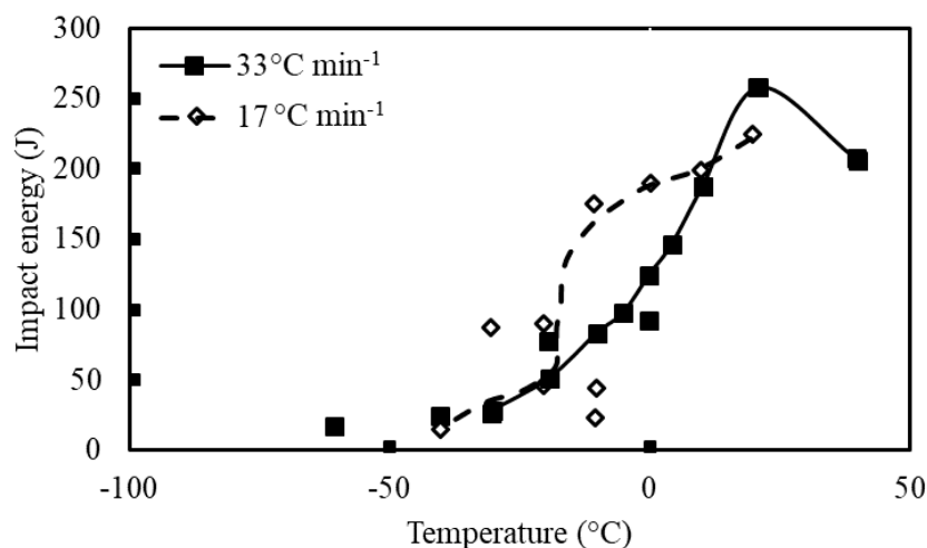
Figure 5-11 Impact energy of the 0.018%Nb steel at both cooling rates ( 33 and 17^{\circ}\text{C min}^{-1} ).
