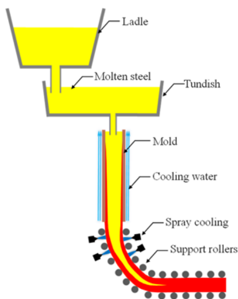
Figure 2-1 Schematic description of the continuous casting process of steel [31].
