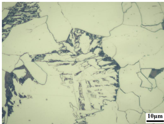
Figure 5-21 A typical optical micrograph of Widmanstätten ferrite in the 0.018%Nb steel at 17°C min -1 .
