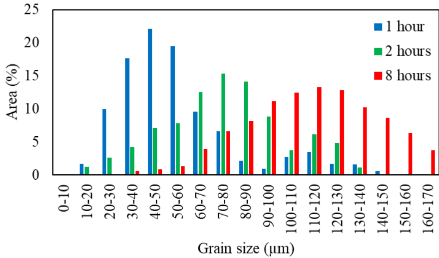
Figure 2-30 (a) Volume fraction of AlN particles after reheating at 1125°C for 1, 2 and 8 hours, (b) prior austenite grain size distribution after reheating at 1125°C for 1, 2 and 8 hours, for the composition: 0.10%C, 0.4%Mn, 0.005%S, 0.3%Si, 0.017%P, 0.016%Al, 0.02%Nb, 0.001%Ti, 0.3%Ni and 0.008%N [114].
