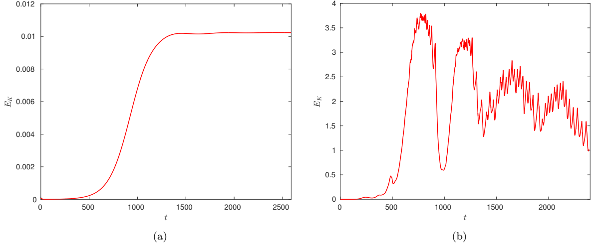
Figure A.6: Temporal evolution of the kinetic energy E_k for (a) \sigma = 0.02 , Ra \approx 625 and (b) \sigma = 0.001 , Ra \approx 12500 .
