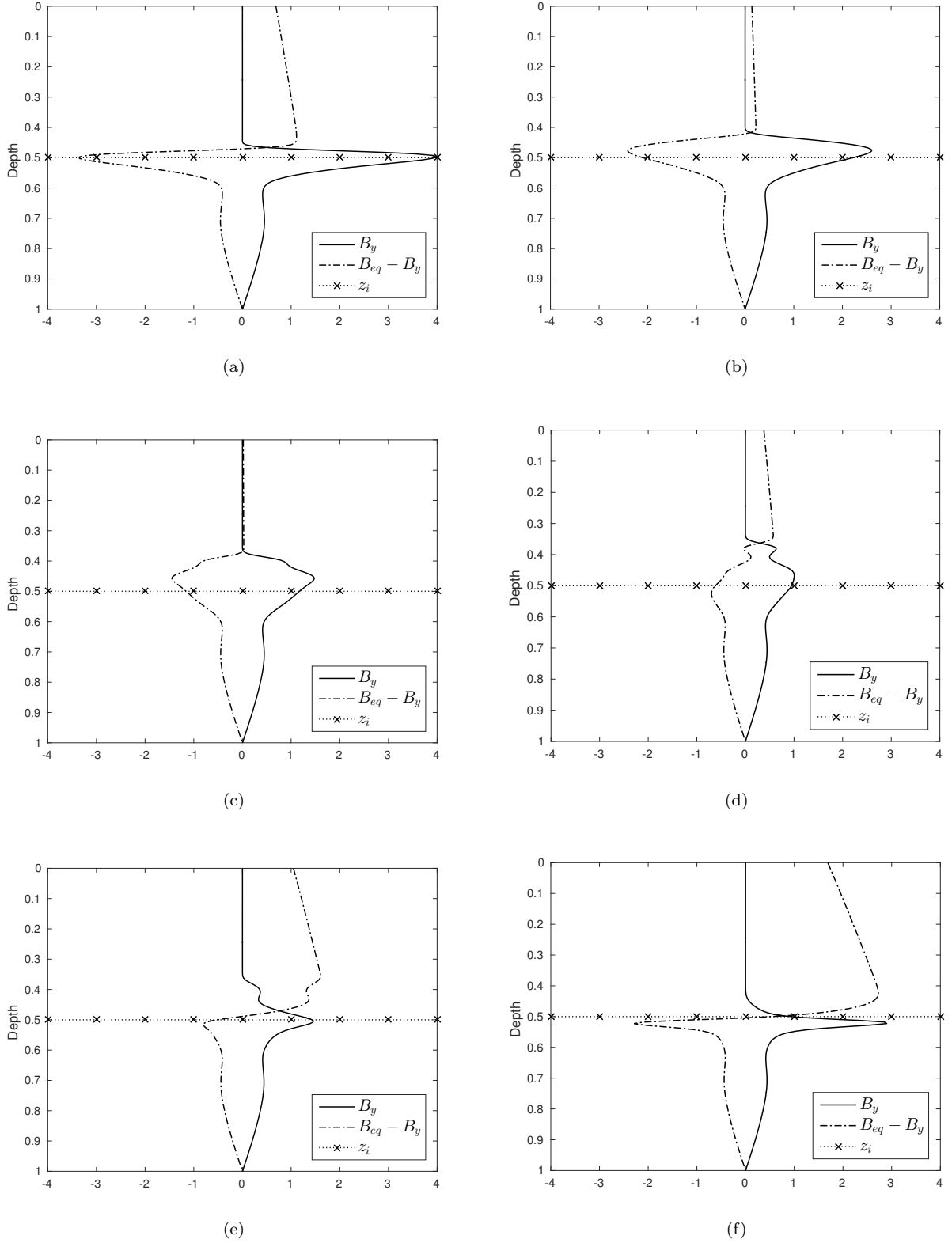
Figure 3.5: The horizontal magnetic field B_y and the difference B_{eq} - B_y vs. depth for a magnetic structure in Case 1, located at x = 0.25 and y = 0 , at times (a) t = 210.8 , (b) t = 211.5 , (c) t = 212.2 , (d) t = 212.9 , (e) t = 213.6 , and (f) t = 214.4 .
