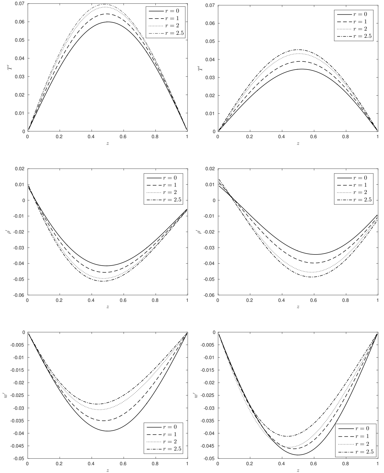
Figure 5.6: Eigenfunctions of the perturbed temperature field (top panel), density (middle panel), and vertical velocity (bottom panel) for polytropic indices m = 0.1 (left) and m = 1 (right), for several r values.
