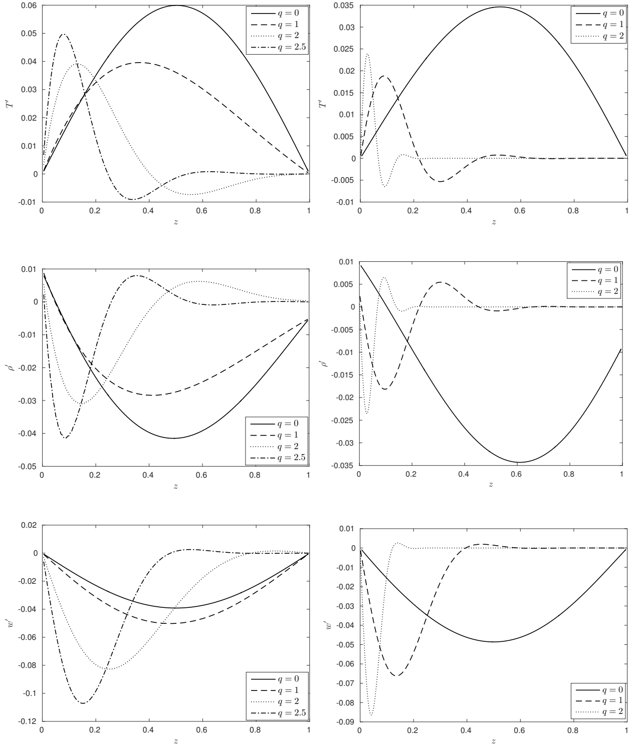
Figure 5.5: Eigenfunctions of the perturbed temperature field (top panel), density (middle panel), and vertical velocity (bottom panel) for polytropic indices m = 0.1 (left) and m = 1 (right), for several q values.
