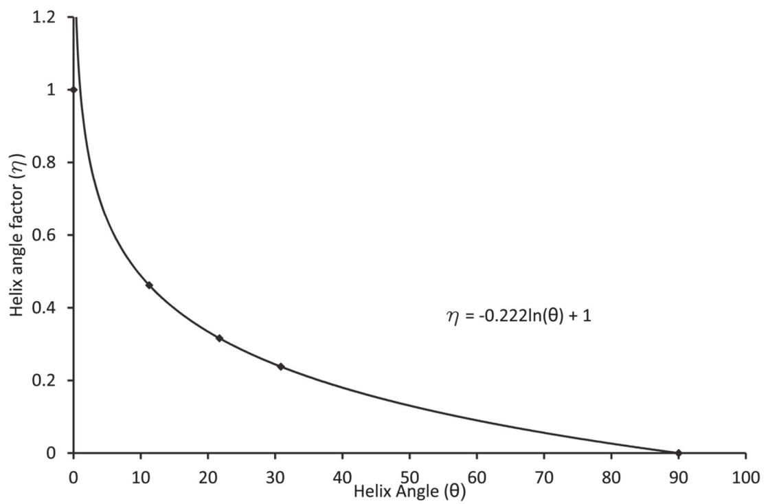
Figure 6.14 Helix angle factor ( \eta ) against the helix angle ( \theta ) for helical ribs.
