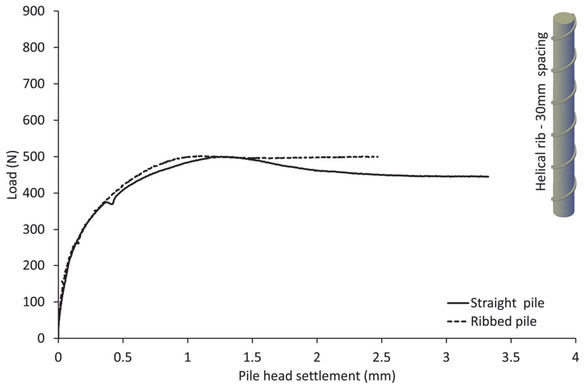
Figure 5.22 Load settlement curve, Test RJG17, helically ribbed pile with 30mm spacing.
