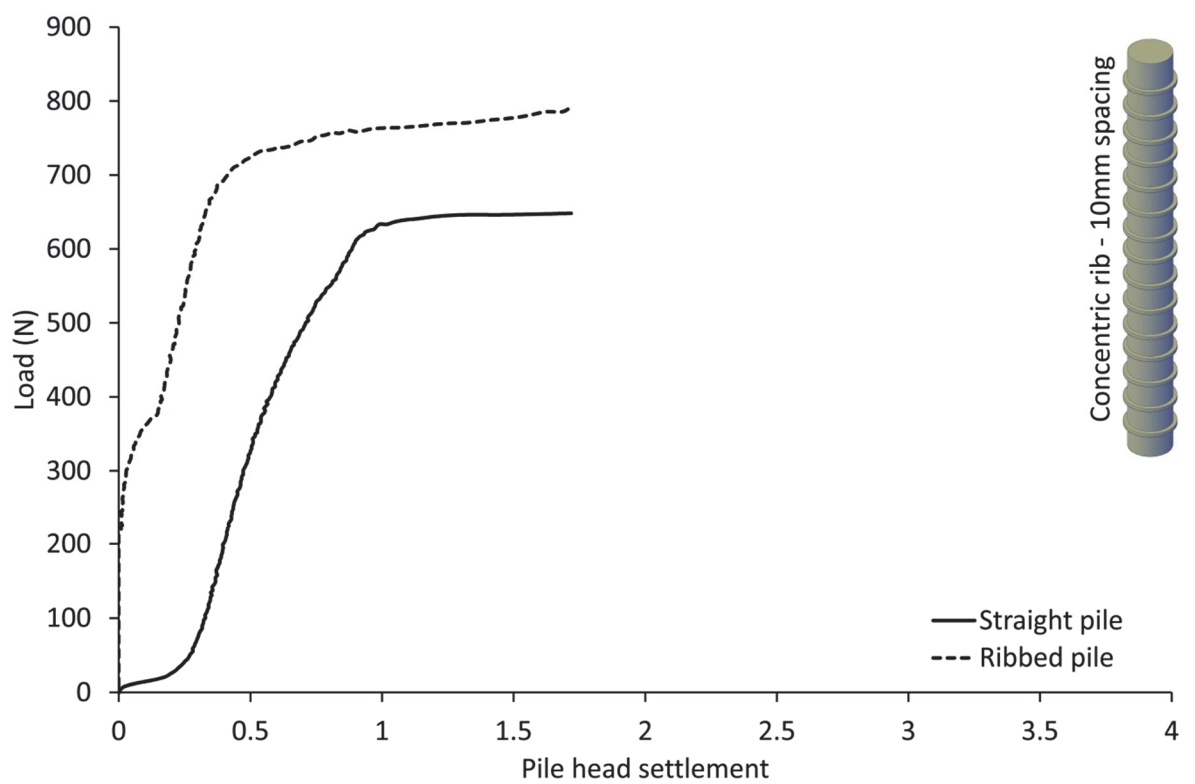
Figure 5.8 Load settlement curve, Test RJG0, concentrically ribbed pile with 10mm spacing using existing test equipment.
