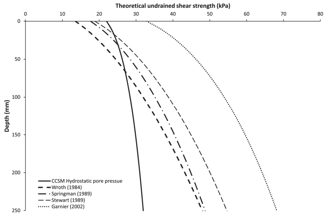
Figure 3.3 Estimated undrained shear strength profile with depth.
