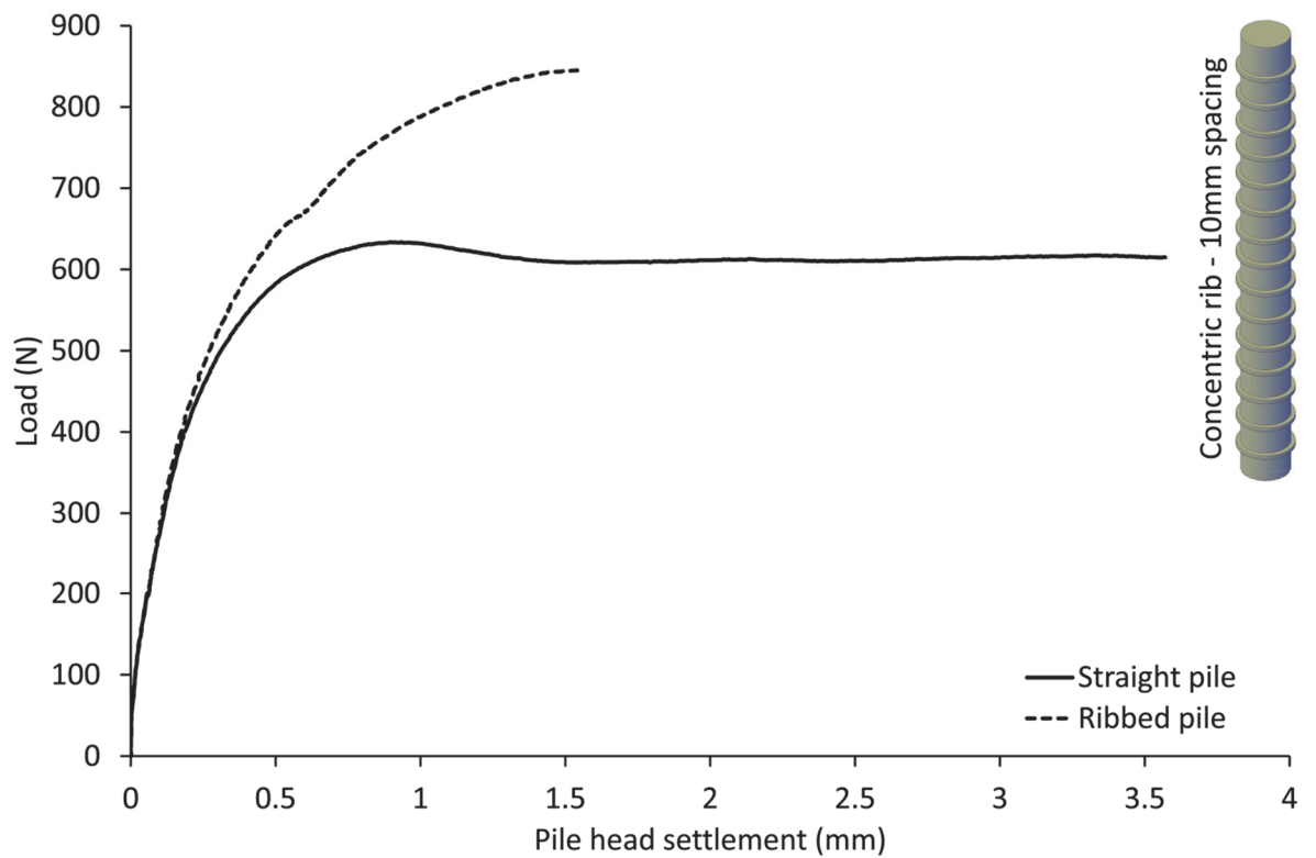
Figure 5.12 Load settlement curve, Test RJG3, concentrically ribbed pile with 10mm spacing.
