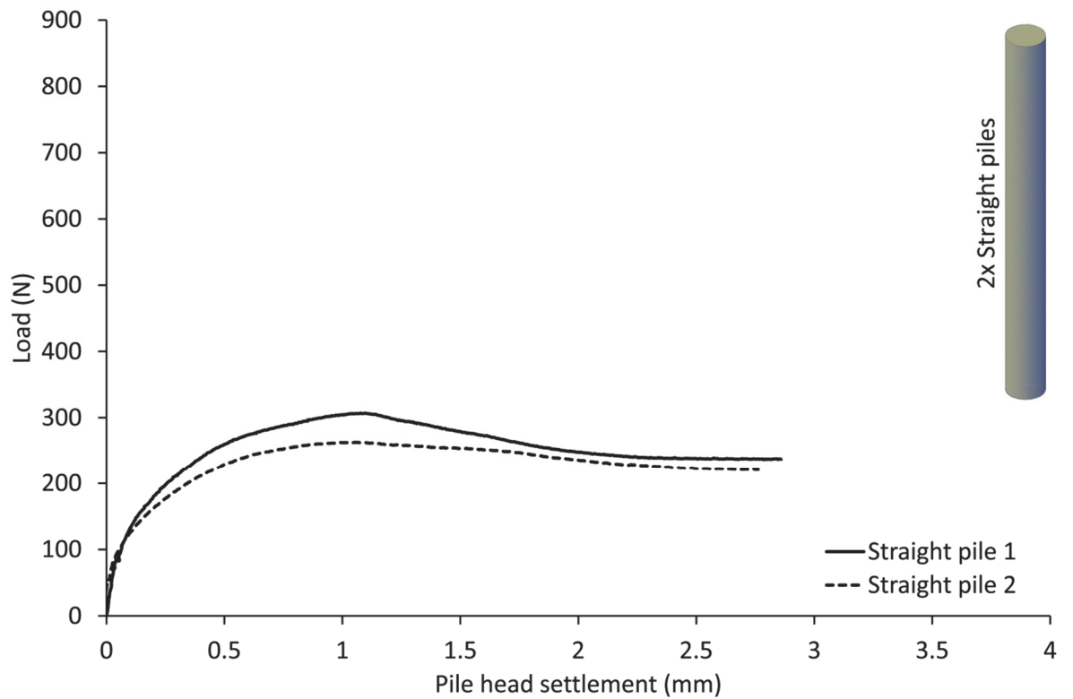
Figure 5.10 Load settlement curve, Test RJG5, 2 straight shafted piles.
