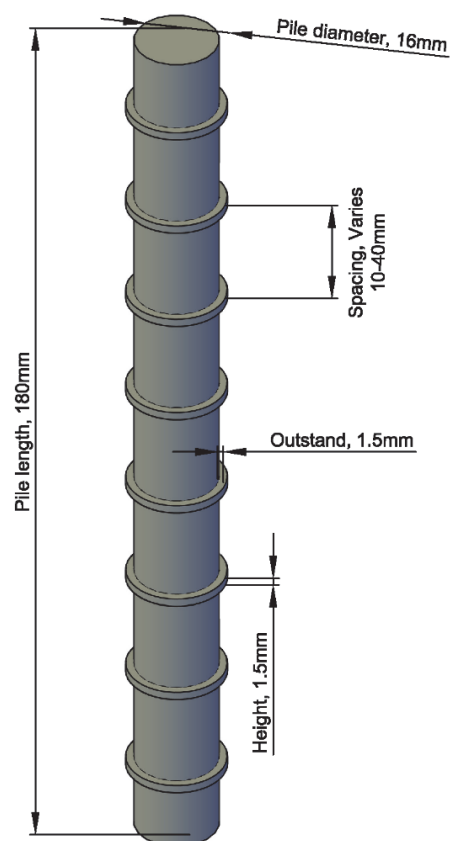
Figure 5.1 Typical pile dimensions.
