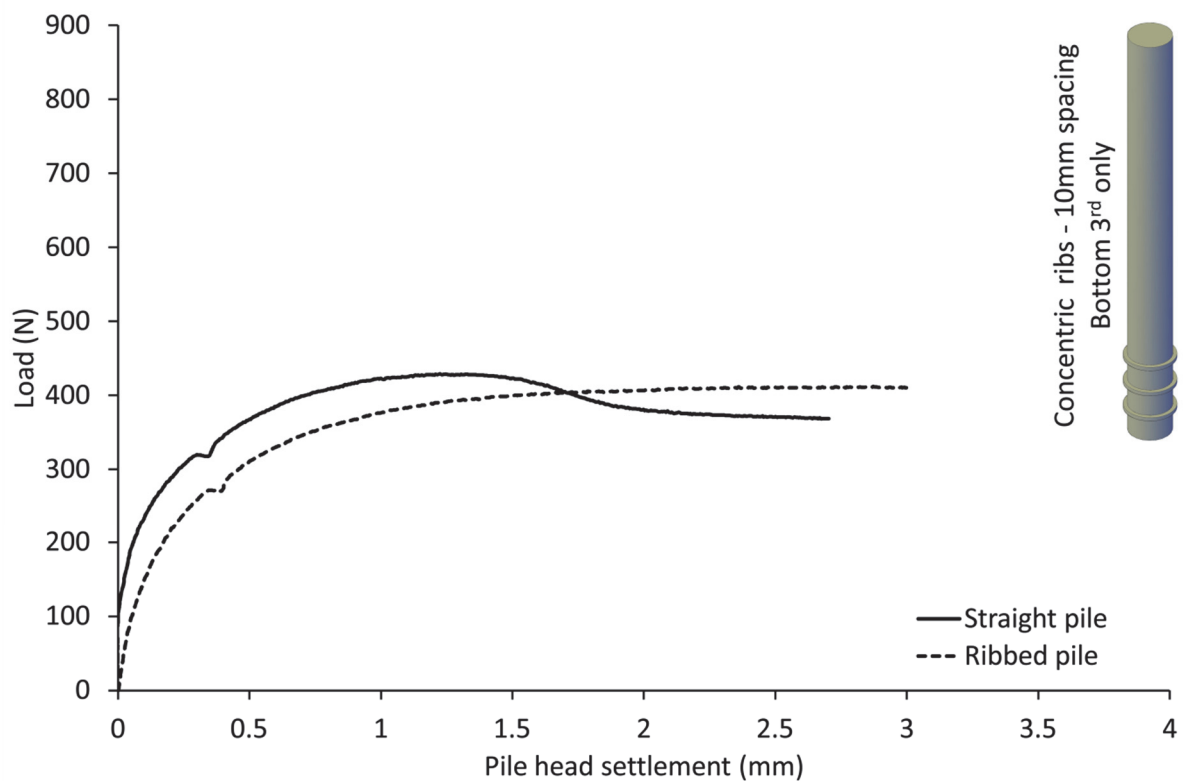
Figure 5.18 Load settlement curve, Test RJG14, concentrically ribbed pile with 10mm spacing with ribs only in bottom third of pile.
