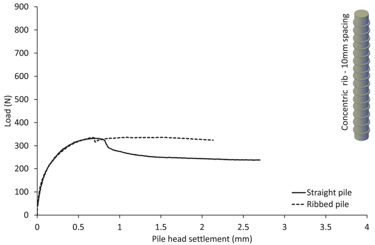
Figure 5.9 Load settlement curve, Test RJG2, concentrically ribbed pile with 10mm spacing.
