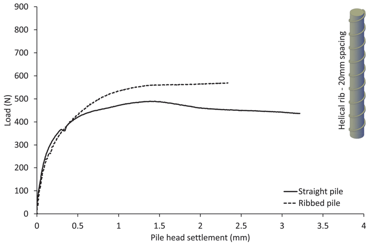
Figure 5.21 Load settlement curve, Test RJG16, helically ribbed pile with 20mm spacing.
