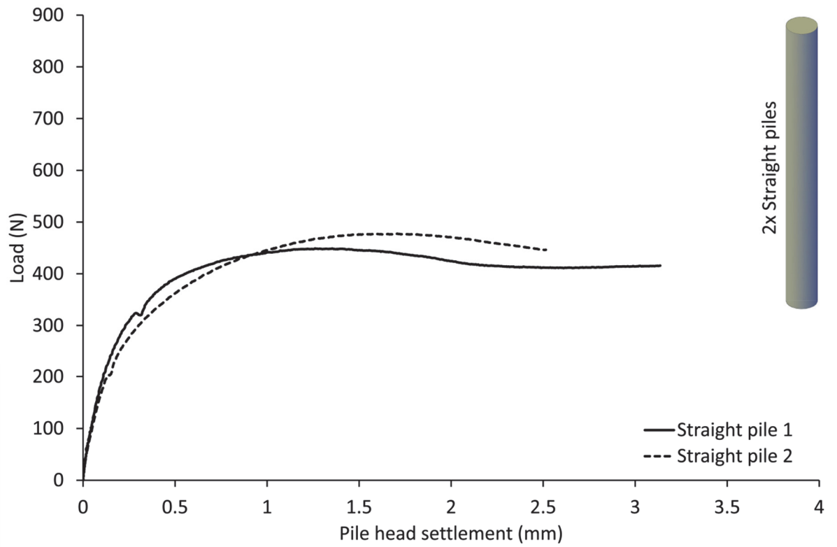
Figure 5.11 Load settlement curve, Test RJG6, 2 straight shafted piles.
