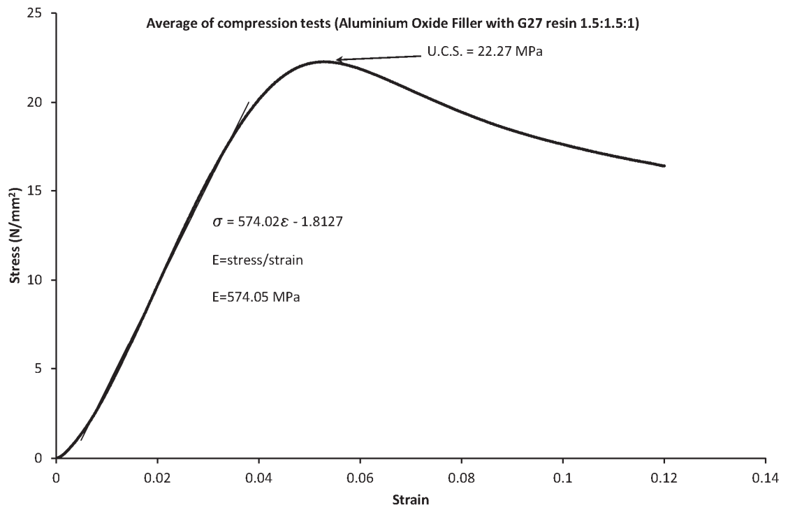
Figure 4.10 Compressive load tests on Sika Biresein G27 resin with Al 2 O 3 filler.
