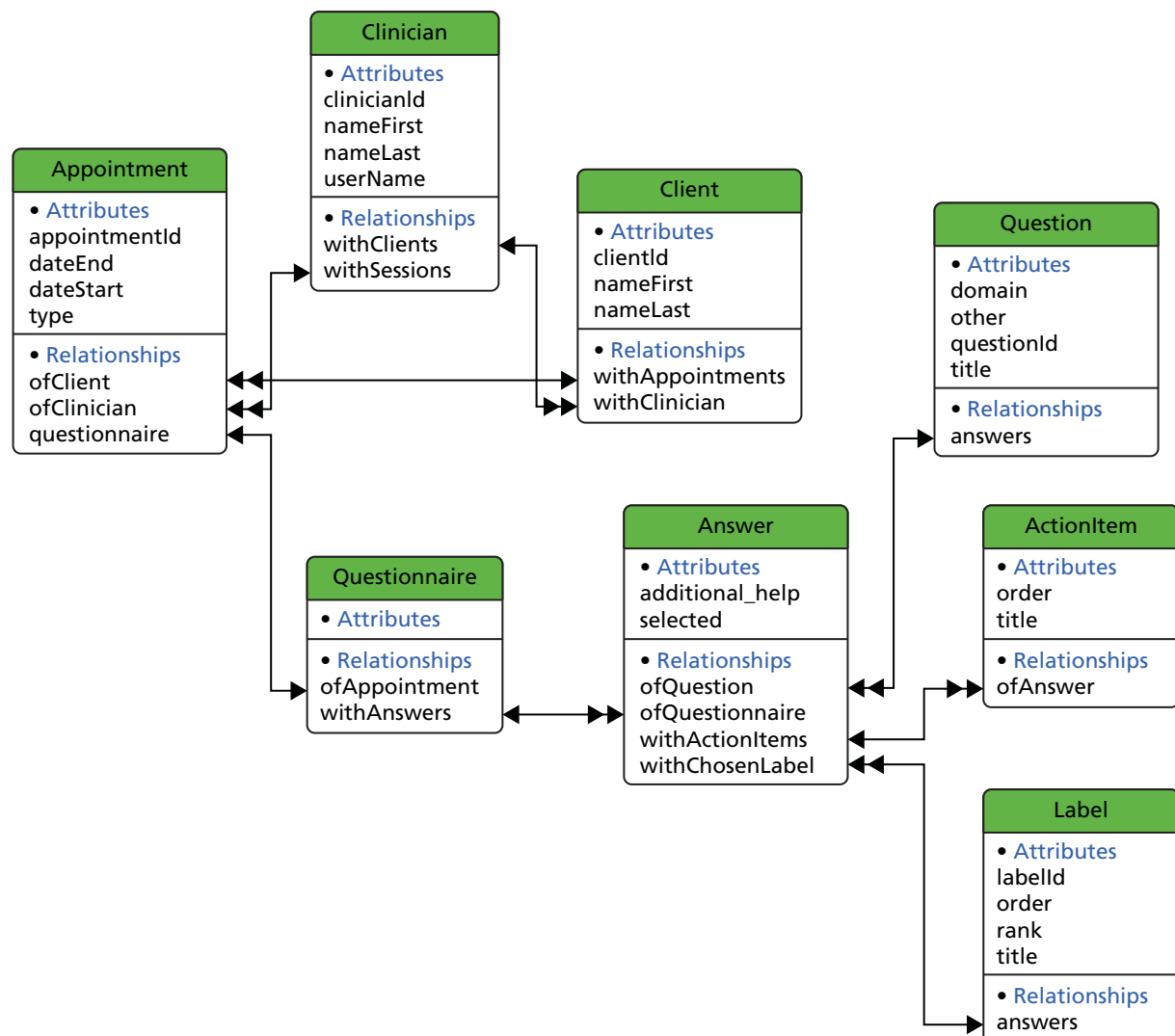
FIGURE 2 Model design of DIALOG based on the Apple Inc. Core Data persistent framework.
