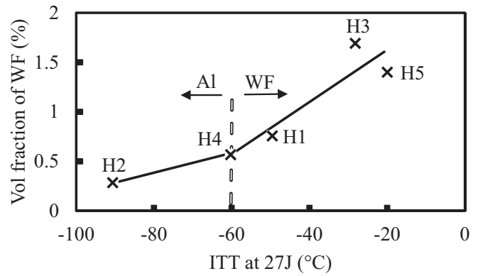
Fig. 13. Apparent influence of Widmanstätten ferrite on the impact behaviour of the hot rolled steels examined. Unfortunately, the effect of WF on impact behaviour is unclear from the literature [22,24]. Bodnar and Hansen [22] as mentioned found 60% WF hardly influenced the impact behaviour of plain C-Mn steels, Fig. 14a whilst Morrison and Preston [24] found it detrimental when produced in Nb containing steels, Fig. 14b.
