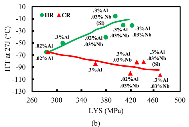
Fig. 16. (a) Impact/strength relationship for presently examined 0.06% C steels. The figures in the brackets are the percentage volume fraction of WF, (b) Impact/strength relationship for the previously examined 15 mm thick plates having 0.1% C, in which an Al addition of 0.3% had been made [4].
