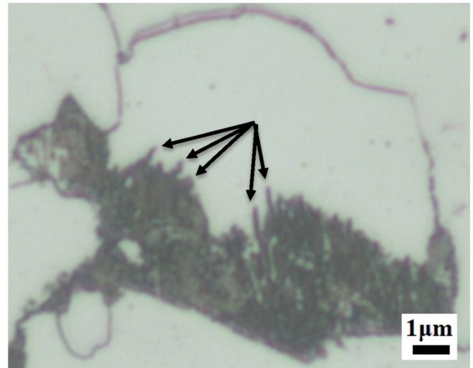
Fig. 10. Bainitic carbides (arrowed) protruding into the ferrite interior in plate H5.
