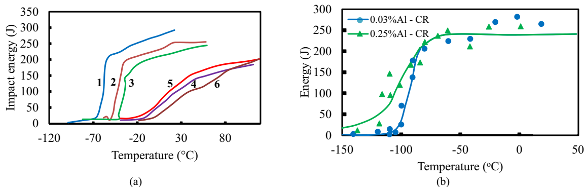
Fig. 1. (a) Influence of 0.3% Al and 0.03% Nb additions on the impact transition curves of hot rolled 15 mm thick, 0.1% C, 1.4% Mn plate [4]. Curve 1, 0.02% Al, curve 2, 0.3% Al, curve 3, 0.02% Al and Nb, curves 4, 5 and 6, 0.3% Al and Nb, (b) ITT curves of control rolled Nb containing steel at two Al levels, 0.03 and 0.25%, (30 mm thick plate) [4].
