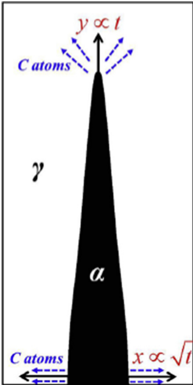
Fig. 12. Growth features of the acicular WF precipitate at the X-axis and Y-axis, where t is the time [15].
