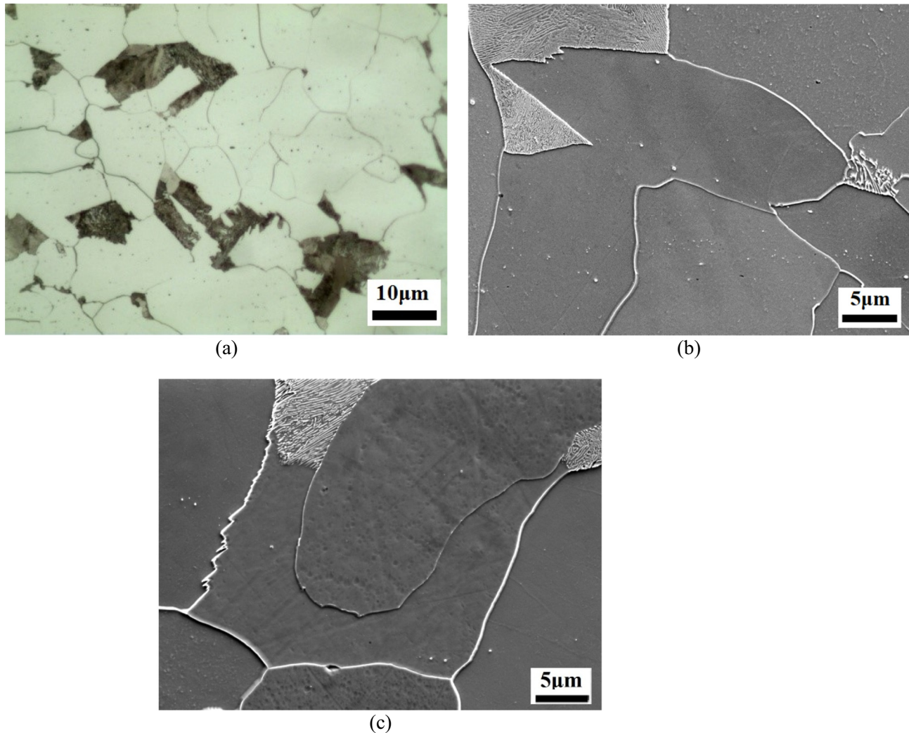
Fig. 4. Control rolled plate C2 having 0.16% Al. Essentially ferrite-pearlite but saw cuts and zig zag boundaries are noticeable indicating the onset of WF formation. The amount of WF was 0.25%. (a) OM (b and c) SEM.
