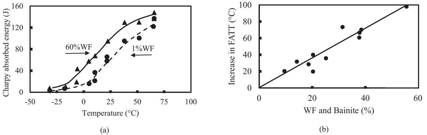
Fig. 14. (a) ITT curves for an 0.2% C, 0.7% Mn steel having the same \gamma grain size of 60 \mu\text{m} cooled at two different cooling rates, 4 and \sim 360 °C/min showing little change in ITTs although WF changes from 1 to 60% [22], (b) Influence of Widmanstätten ferrite or bainite on the ITT of a Nb containing steel. 1% WF increases ITT by 2 °C [24].
