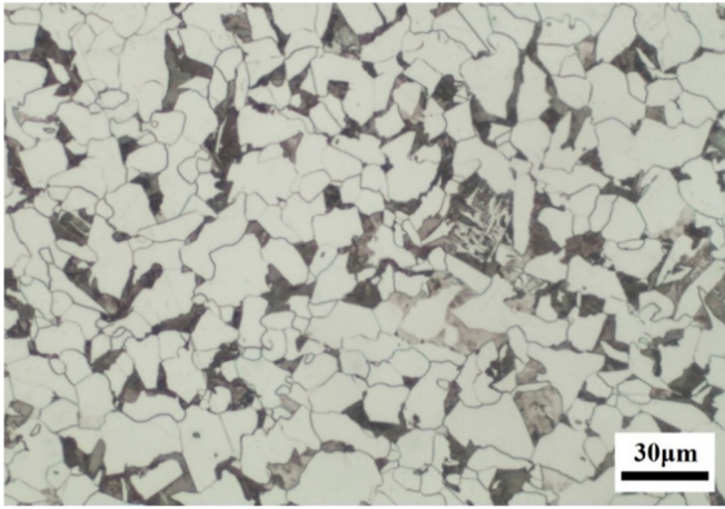
Fig. 5. WF is still present in the more slowly cooled low Al (0.02%) thicker 30 mm plate, H4, (0.6% WF) but MA was not observed.
