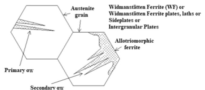
Fig. 11. Various forms of WF [14].
