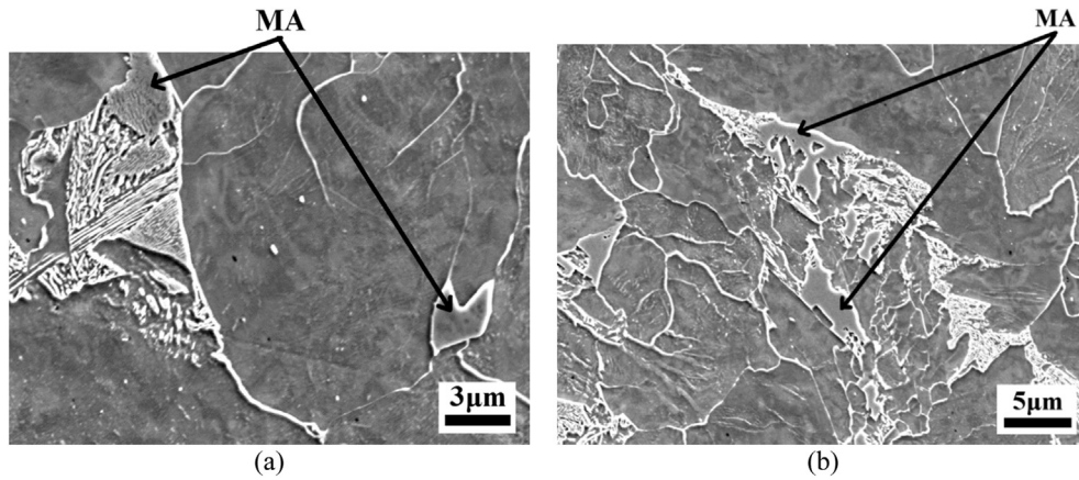
Fig. 7. (a and b) Control rolled high Al/Nb containing steel, C3 showing examples of regions with WF (1.3%) and MA. The plate thickness is 15 mm.
