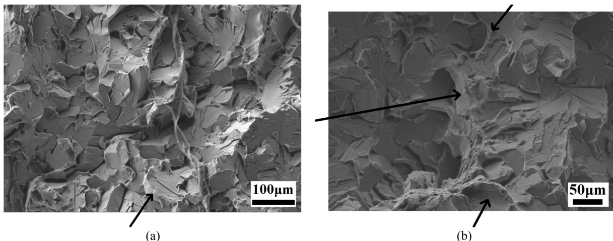
Fig. 8. Fracture surface of the hot rolled 30 mm thick plate (a) Nb/Al, H5 tested at −40 °C, and (b) low Al, H4 tested at −70 °C.
