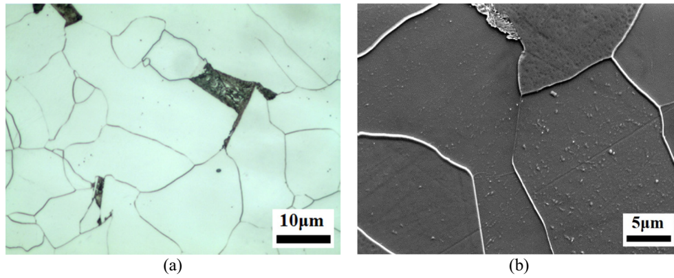
Fig. 3. Hot rolled microstructure of plate H1, the base plain C-Mn steel, (0.02% Al) showing evidence of a small amount of WF (0.75% WF) but no MA. (a) OM (b) SEM.
