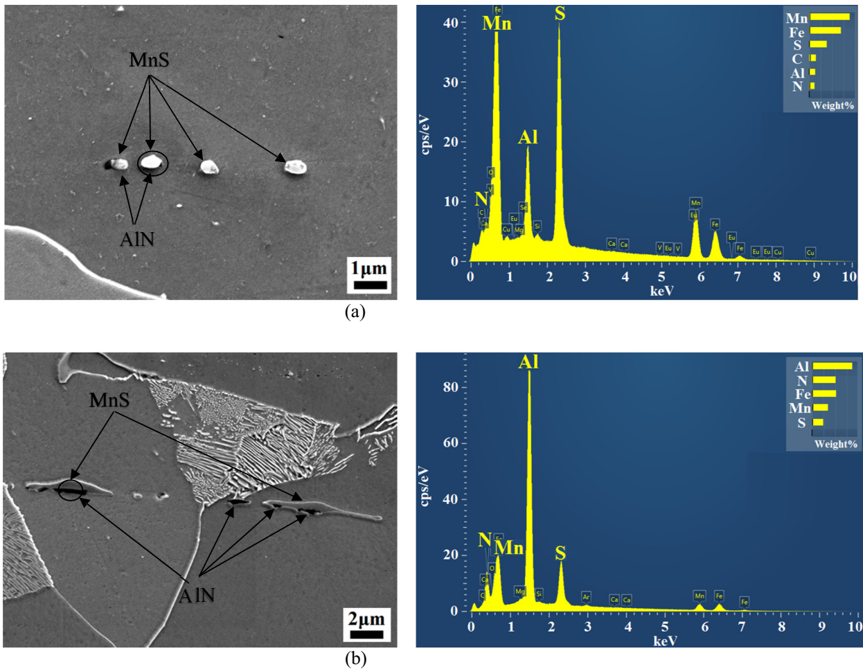
Fig. 9. Typical particles and their average analysis (a) Particles were either manganese sulphides and AlN, or (b) Elongated MnS inclusions combined with AlN. The micrographs (a) and (b) were taken from plate C2, AlN shows up as black and MnS as grey.
