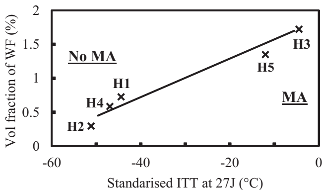
Fig. 15. WF, (volume fraction %) vs 27J ITT °C, standardised to d^{-1/2} = 6 \text{ mm}^{-1/2} , \Delta p = 0 and the absence of any benefit from Al for the hot rolled plates.
