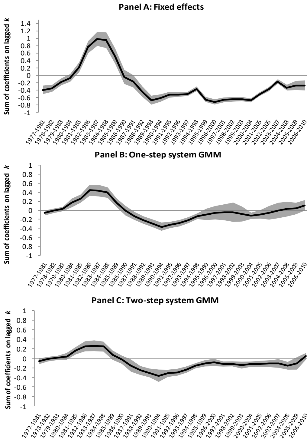
Figure 5.4: Estimated effect of k on ROE 1977-2010
