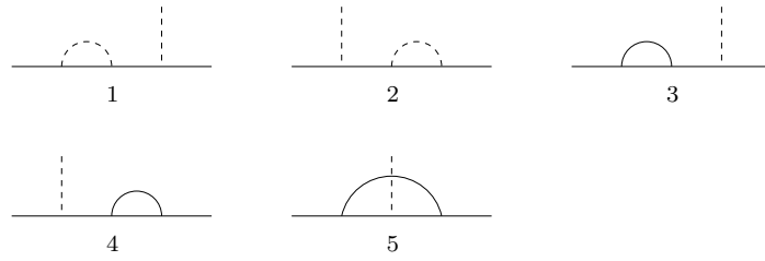
Figure 1.32: Half diagrams in T((0, 1))
