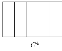
Figure 1.10: Basis elements of TL_4(\delta) with 4 lines
