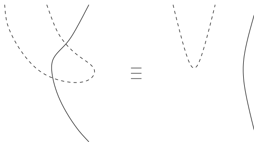
Figure 1.20: Both are equivalent
