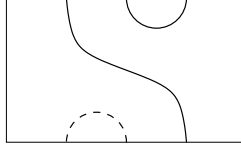
Figure 1.34: Basis element of TL_3^2(\delta_R, \delta_G)
