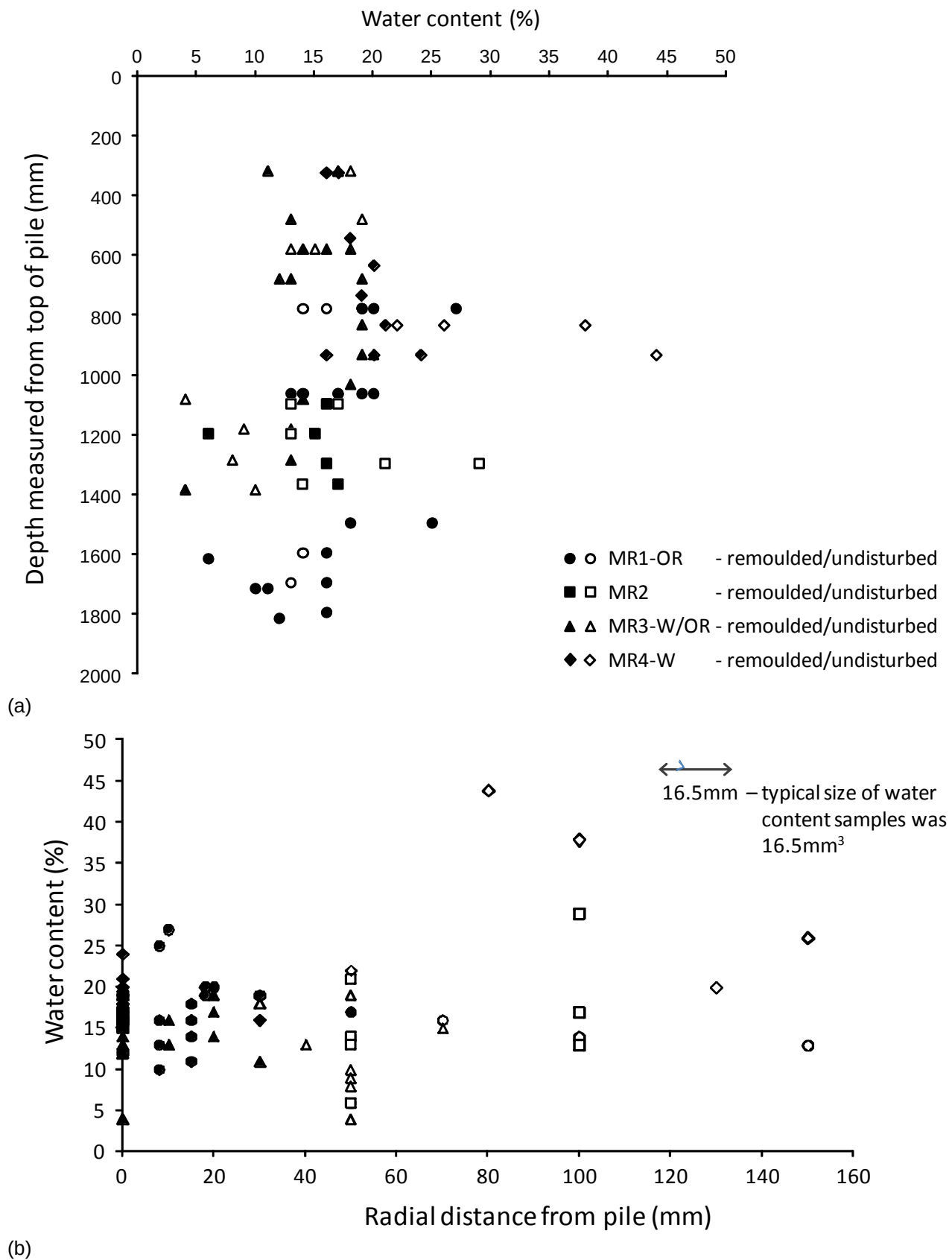
Figure 12 Variation in water content with (a) depth and (b) radial distance from the pile. Data from all piles, remoulded and undisturbed soil
