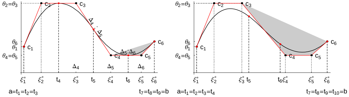
Fig. 1. Quadratic (left panel) and cubic (right panel) functional spline curves \mathbf{Q}^*(t) and their control polygons \mathbf{C}_Q .
