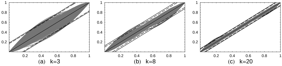
Fig. 2. Graphs of 1000 simulations of \sum_{i=1}^p \xi_i N_{i,3}(t) , with t_{k,3} according to (25) and estimates of \hat{e}_{0.95} and \hat{\epsilon}_{0.95} for: (a) p = 6 ( k = 3 ), \hat{e}_{0.95} = 0.17 , \hat{\epsilon}_{0.95} = 0.18 ; (b) p = 11 ( k = 8 ), \hat{e}_{0.95} = 0.10 , \hat{\epsilon}_{0.95} = 0.12 ; (c) p = 23 ( k = 20 ), \hat{e}_{0.95} = 0.05 , \hat{\epsilon}_{0.95} = 0.07 .
