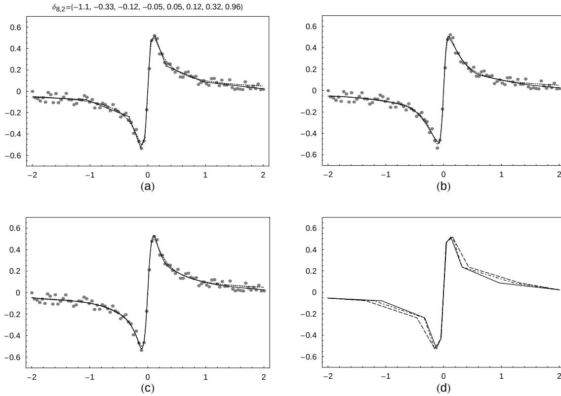
Fig. 3. The final GeD spline fits: (a) linear; (b) quadratic; (c) cubic; (d) graphs of \hat{f}(\delta_{8,2}, \hat{\alpha}; x) - the solid line, \mathbf{C}f_{(\bar{t}_{8-(n-2),n}, \hat{\alpha}; x)} - the dot-dashed line and \mathbf{C}f_{(\bar{t}_{8-(n-2),n}, \hat{\alpha}; x)} - the dashed line; The dotted curve in (a), (b), (c) is the true function.
