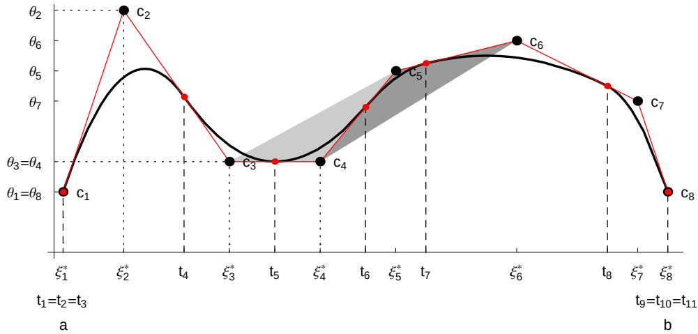
Fig. 1. A quadratic, functional spline regression curve Q^*(t) and its control polygon C_{Q^*} .
