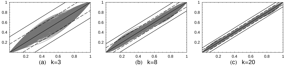
Fig. 2. Graphs of 1000 simulations of \sum_{i=1}^p \xi_i N_{i,n}(t) , with \Delta_{k,3} according to (13) and estimates of \hat{\delta}_{0.95}^{\max} and \hat{b}_{0.95}^{\max} for (a) p = 6 ( k = 3 ), \hat{\delta}_{0.95}^{\max} = 0.16 , \hat{b}_{0.95}^{\max} = 0.31 ; (b) p = 11 ( k = 8 ), \hat{\delta}_{0.95}^{\max} = 0.09 , \hat{b}_{0.95}^{\max} = 0.17 ; (c) p = 23 ( k = 20 ), \hat{\delta}_{0.95}^{\max} = 0.05 , \hat{b}_{0.95}^{\max} = 0.09 .
