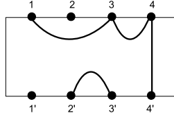
FIGURE 2.1: A diagrammatic representation of a partition from \mathcal{P}_{\underline{4} \cup \underline{4}'} .
