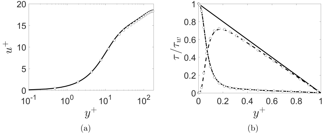
Figure 2.4: (a) Mean velocity profile in wall units. (b) The total shear stress (solid line), decomposed in the viscous stress (dash-dotted line) and Reynolds shear stress (dashed line) obtained from the simulation. The circles in both the plots are used for the results by Moser et al. (1999).
