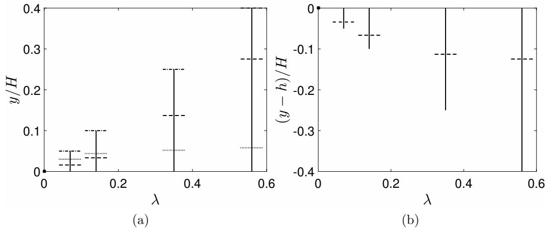
Figure 4.2: (a) Mean locations of the two inflection points and of the virtual origin along the canopy stem (virtual origin: --- ; inner inflection point: .....; outer inflection point: - · -). (b) Location of the virtual origin in a reference system whose zero is set at the canopy tip. Note that the small dot on the left of the horizontal axis (bottom in (a) and top in (b)) represents a flow on a smooth surface (i.e. no-canopy).
