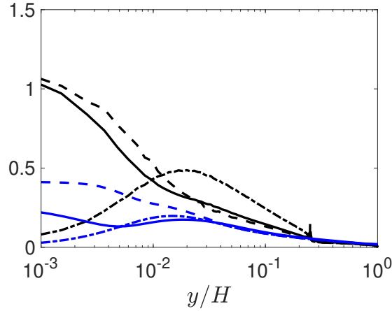
Figure 3.6: Black lines refer to the actual canopy simulation while the blue ones are taken from the channel flow data of Hoyas and Jiménez (2008). Solid line \omega'_{x,rms}^+ , dashed-dotted line \omega'_{y,rms}^+ , dashed line \omega'_{z,rms}^+ . The wall units are based on the local friction velocity u_{\tau,l} .
