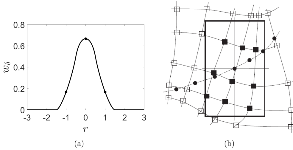
Figure 2.5: (a) Kernel function proposed by Roma et al. (1999). (b) Taken from Pinelli et al. (2010). The black rectangle is the cage around one of the Lagrangian points, shown as dots. The squares represents grid points, and the black ones are the grid points falling within the cage.
