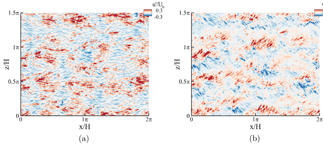
Figure 3.7: Panel (a): contours of instantaneous streamwise velocity fluctuations inside the canopy, on a plane located at y/H = 0.02 . Panel (b): spanwise velocity fluctuations on the same plane as (a)
