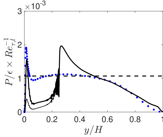
Figure 3.4: Turbulent kinetic energy production to dissipation ratio. Thick solid line: ratio normalised with the local friction Reynolds number, defined as Re_{\tau,l} = u_{\tau,l}H/\nu , where u_{\tau,l} is as given in (3.8); Thin solid line: same quantity normalised with the outer friction Reynolds number; Dashed horizontal line: production to dissipation equilibrium condition (i.e. 1/Re_{\tau,l} ); Blue dotted symbols are plane turbulent channel flow data at Re_{\tau} = 950 (Hoyas and Jiménez, 2008).
