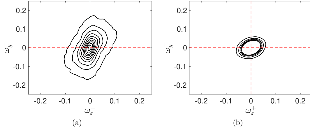
Figure 3.12: Joint probability density function of \omega_x and \omega_y . Panel (a), on the left is computed on a x - z plane at y/H = 0.18 ( y_{out}^+ = 48 ); Panel (b) is for a x - z plane at y/H = 0.63 ( y_{out}^+ = 541 ). The vorticity components are normalised with \nu/u_{\tau,out}^2 . Range and increment in (a) are [0:5:50] , in (b) [0:10:50] . Red dashed lines are the Cartesian axes through the origin.
