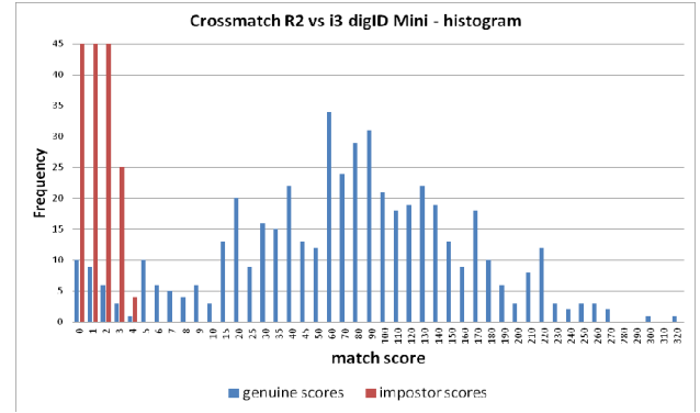
Figure 4: The histogram of the DDMG and DDMI scores for the Cross Match Guardian R2 vs. i3 digID Mini. The frequency of the DDMI scores in the 0-1 range is 19,889, for 1-2 is 4,024 and for 2-3 is 229.
