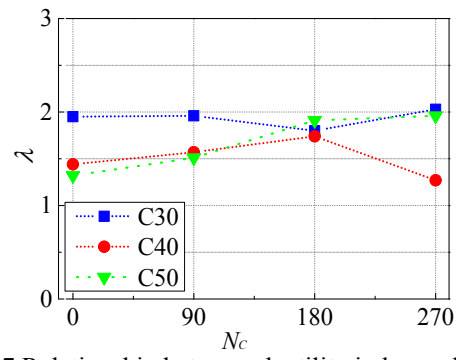
Fig. 7 Relationship between ductility index and N_c
