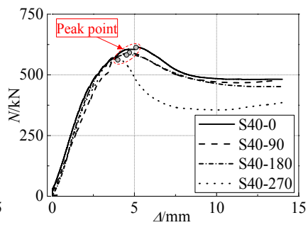
(b) C40 specimens
