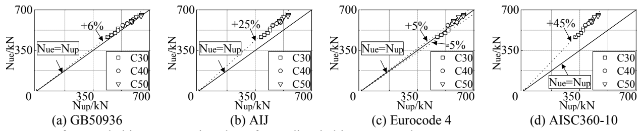
Fig. 13 Comparisons between tested and predicted ultimate strength of CFST columns
