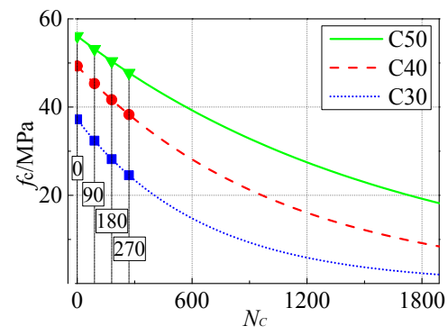
Fig. 15 Strength degradation of core concrete
