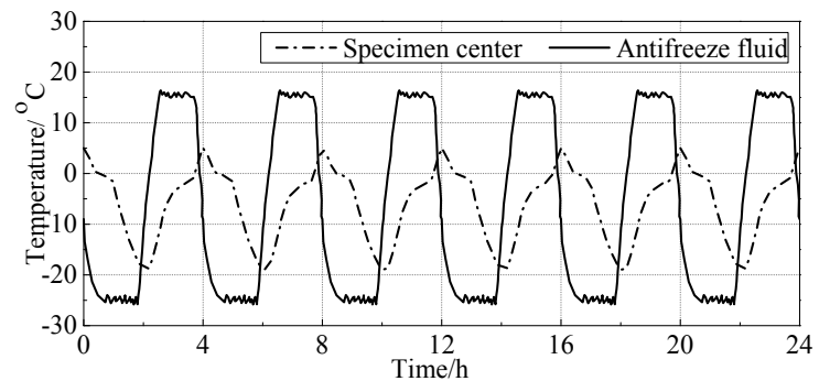
Fig. 2 Freeze-thaw cycles within 24 hours
