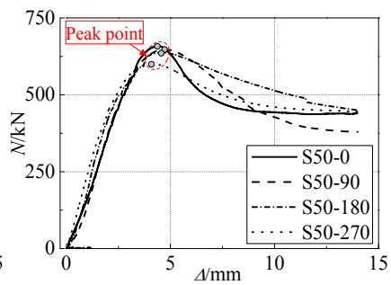
(b) C50 specimens
