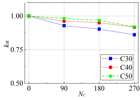
Fig. 11 Influence of N_c and concrete grade on k_{sr}
