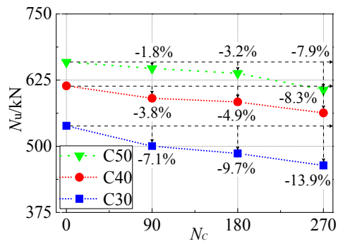
(a) Ultimate strength
