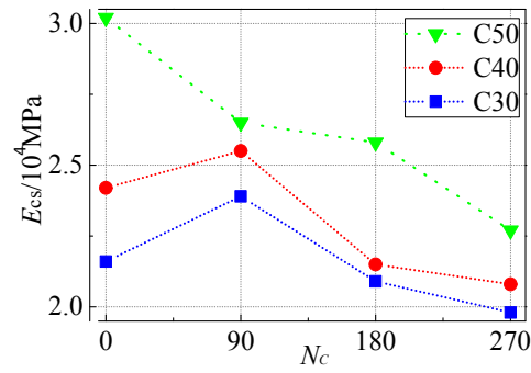
(c) Elastic modulus
