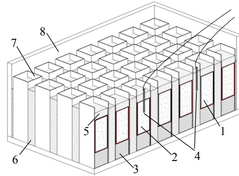
(b) Schematic diagram of equipment and specimens
