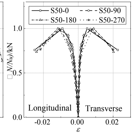
(b) C50 specimens
