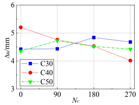
(b) Ultimate displacement
