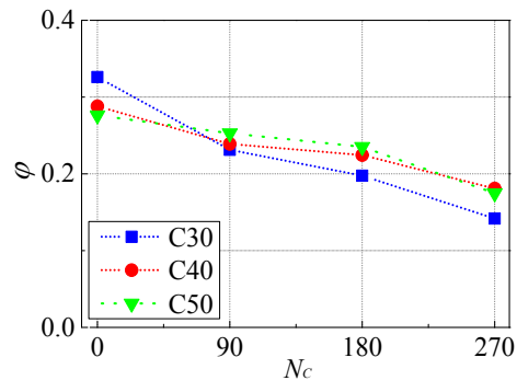
Fig. 10 Relationship between \varphi and N_c
