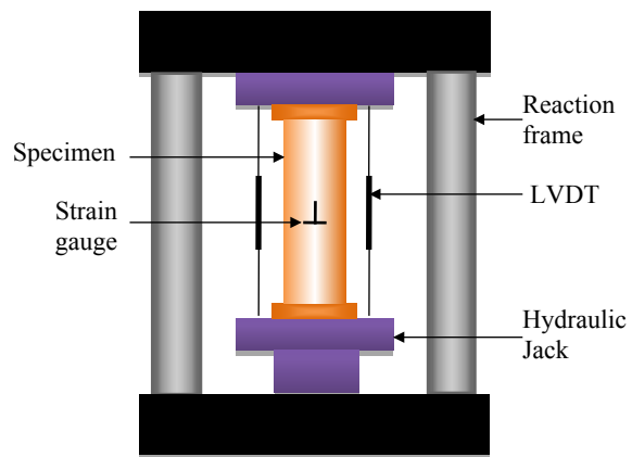
(a) Test setup
