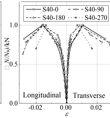
(b) C40 specimens
