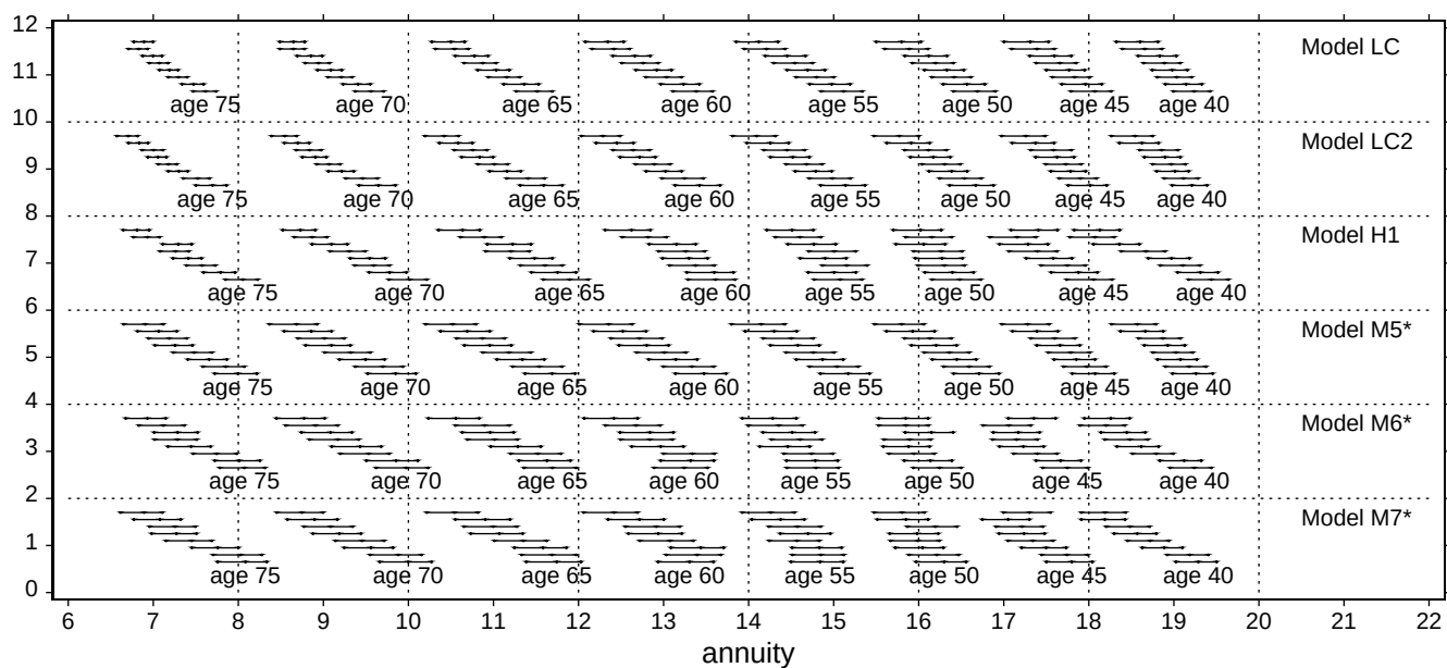
Fig 15a. USA male 1961-2006 mortality experience, age range 20-89. Evolving 1993(02)05,06 life expectancy & 4% annuity prediction intervals.
