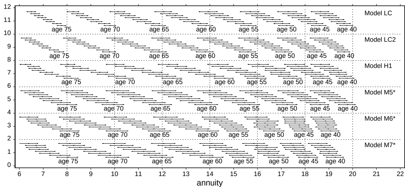
Fig 14a. EW male 1961-2007 mortality experience, age range 20-89. Evolving 1993(02)07 life expectancy & 4% annuity prediction intervals.
