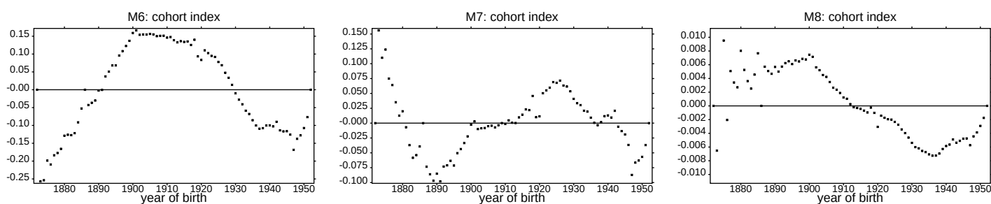
Models M6-M8: year-of-birth indices
