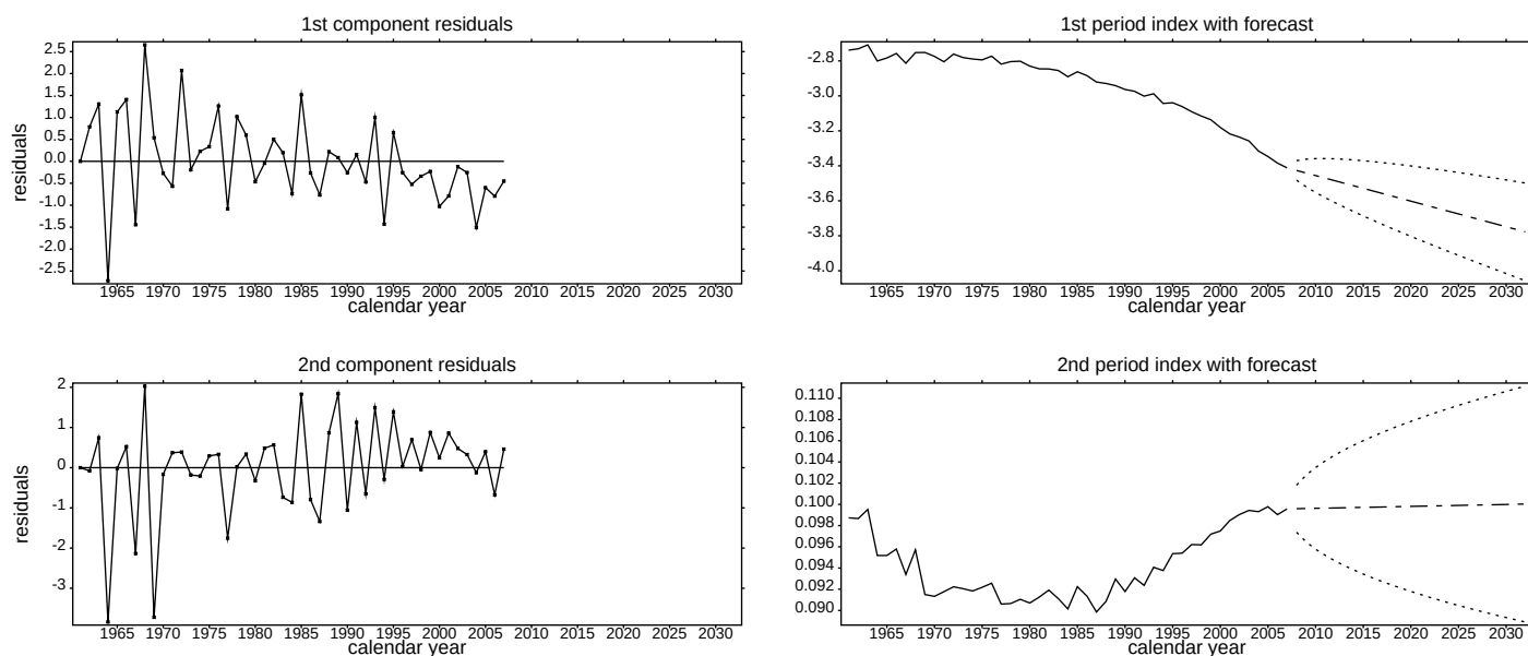
Model M8: period indices bi-variate random walk
