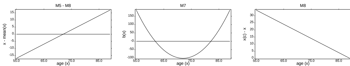
Models M5-M8: age modulating functions
