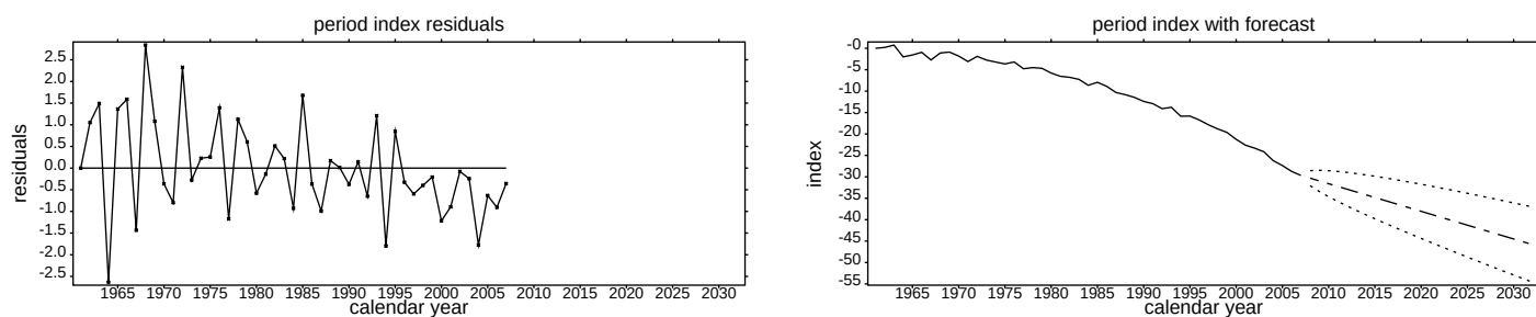
Model LC: period index random walk
