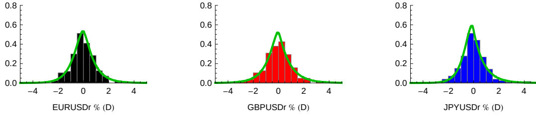
Fig. 7 Marginal LG densities fitted to (histograms of) historic daily log returns of the exchange rates of EUR/USD, GBP/USD and JPY/USD.
