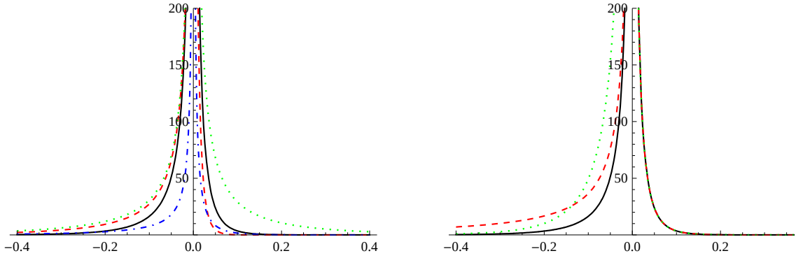
Fig. 1 left panel: Lévy measure of a VG process for the following four sets of parameters \theta = -0.29 , \sigma = 0.19 , \nu = 0.25 (solid line); \theta = -0.99 , \sigma = 0.19 , \nu = 0.25 , (dashed); \theta = -0.29 , \sigma = 0.99 , \nu = 0.25 (dotted) and \theta = -0.29 , \sigma = 0.19 , \nu = 0.95 (dot-dashed); right panel: The LG Lévy measure for \lambda = 1 , and the following three sets of parameters \delta_0 = -0.11 , \delta_1 = 0.04 , \alpha_0 = \alpha_1 = 3.99 (solid line); \delta_0 = -1.13 , \delta_1 = 0.04 , \alpha_0 = \alpha_1 = 3.99 (dashed); and \delta_0 = -0.11 , \delta_1 = 0.04 , \alpha_0 = 11.98 , \alpha_1 = 3.99 (dotted);
