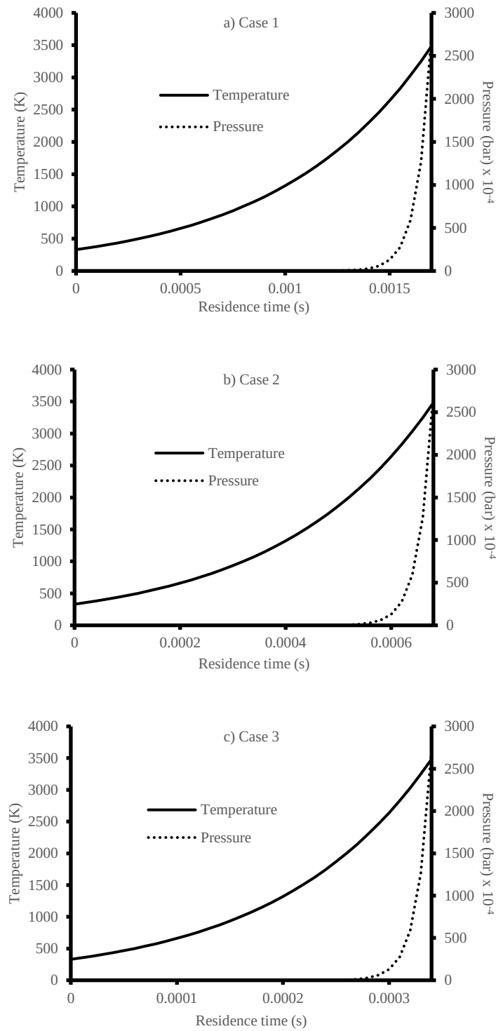
Figure 9.2.1 Polytropic temperature and pressure profiles for the three simulations
