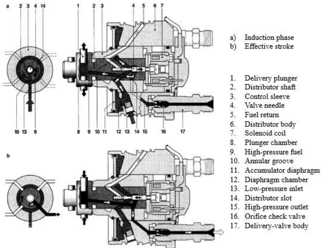
Figure 2.2.5 Cross section view of distributor radial-piston pump [45]
