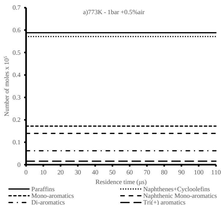
Figure 9.1.3 Variation in number of moles for isotropic profile of major components in the surrogate diesel fuel with 0.5% air addition
