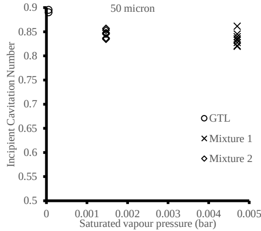
Figure 4.1.14 Incipient cavitation number for all three fuels at 50 \mu m needle lift – acrylic model version 2
