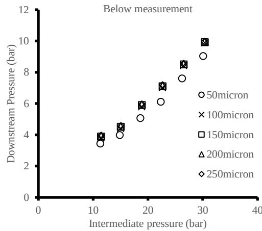
Figure 4.1.8 Below measurements for acrylic model version 1 with paraffinic model diesel using estimated intermediate pressure
