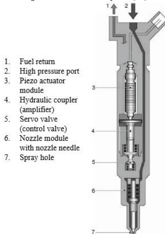
Figure 2.2.8 Piezo injector [42]
