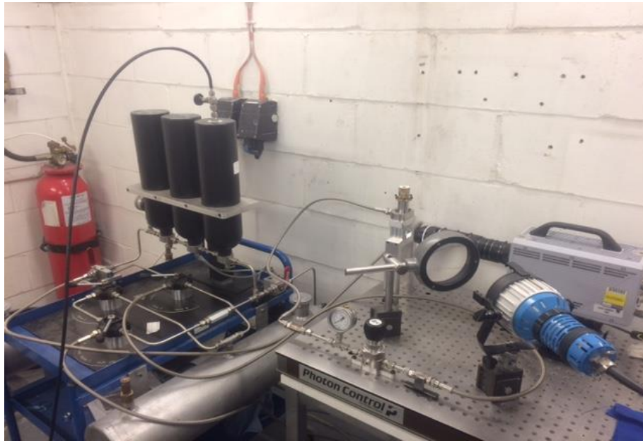
Figure 3.3.2 Experimental setup of low pressure characterisation test
