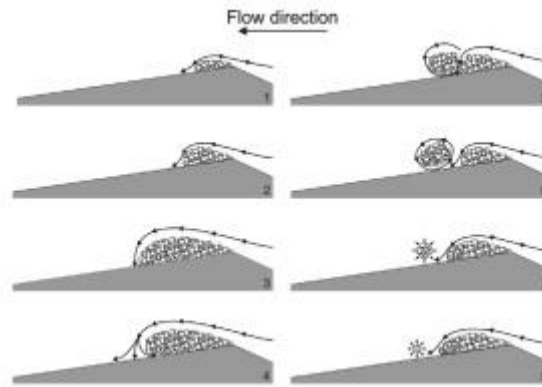
Figure 2.3.1 Developed hydrodynamic cavitation [62]
