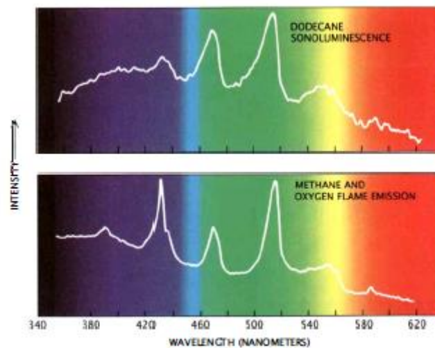
Figure 2.3.4 Comparison of spectra produced by sonoluminescence of dodecane (top) and the combustion of methane (bottom) [14]
