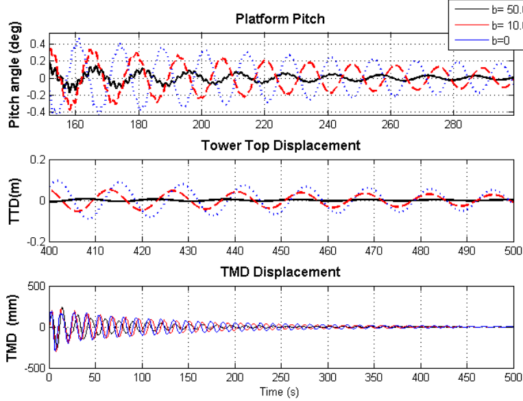
Fig. 5: Comparison between system response with a TMD (blue dotted, TMDI with inertance b=10.000 (red dash) and TMDI with inertance b=50.000 (black solid) in the nacelle.
