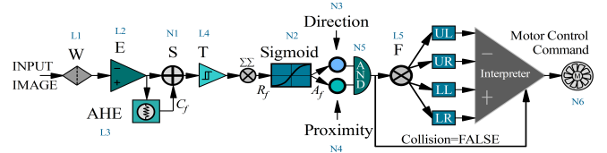
Fig. 1. Schematic illustration of Furcated Luminance-Difference Processing (FLDP) model. The proposed architecture consists of 5 layers (L1,L2,...,L5) of processing namely, linear time-invariant filter (W), excitation (E), adaptive histogram equalization (AHE), threshold (T), and furcation (F). Followed by 6 single processing nodes (N1,N2,...,N6) namely, the direction detector, depth estimator, summation, sigmoid transformer, AND logic gate, and motor control command generator node.
