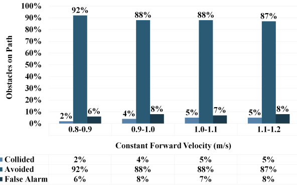
Fig. 14. Schematic illustration of detection errors. A graph of percentage obstacles detected versus linear forward velocity of the robot (8 tests per velocity range) is plotted to represent successful/unsuccessful collision alarms against false alarms for the afore described collision scenarios.
