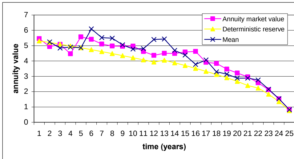
Figure 4: Comparison of the “historical annuity market values” with the mathematical reserves and the annuity fair values calculated using the CIR model.
