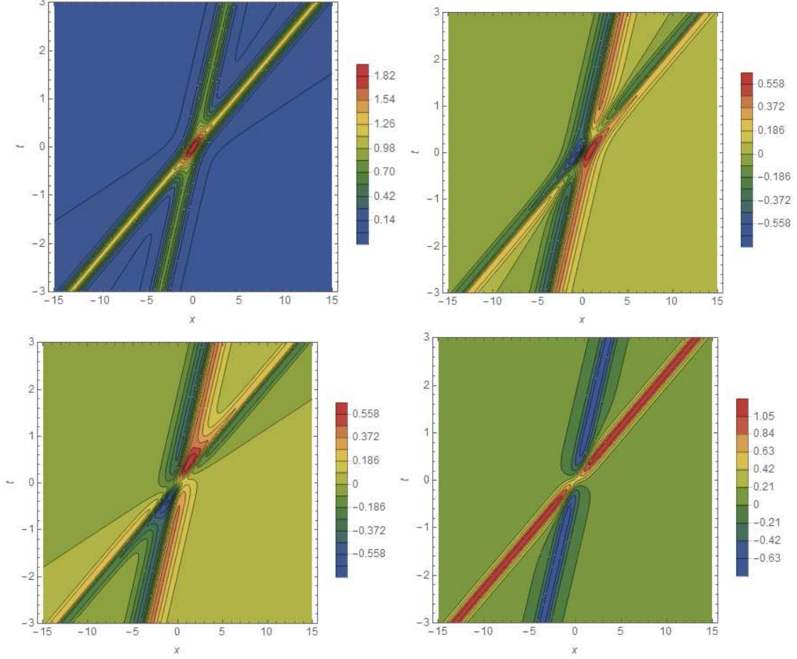
Figure 3: A fast bright soliton overtaking a slower bright soliton in the canonical component functions p , q , r and s (clockwise starting in the top left corner) for the one-soliton solution \hat{u}_{\theta,\phi;\alpha,\beta} to the bicomplex KdV equation (2.16) with \mathcal{PT}_{ij} -symmetry for \alpha = 2.1 , \beta = 1.1 , \theta = 0.6 and \phi = 1.75 .
