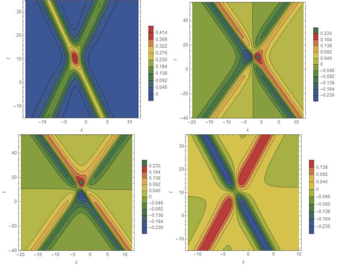
Figure 2: Head-on collision of a bright soliton with a dark soliton in the canonical components p , q , r , s (clockwise starting in the top left corner) for the one-soliton solution h_{\rho,\theta,\phi,\chi;\alpha} to the bicomplex KdV equation (2.16) with broken \mathcal{PT} -symmetry for \alpha = 0.5 , \rho = 1.3 , \theta = 0.1 , \phi = 2.0 and \chi = 1.3 . Time is running vertically, space horizontally and contours of the amplitudes are colour-coded indicated as in the legends.
