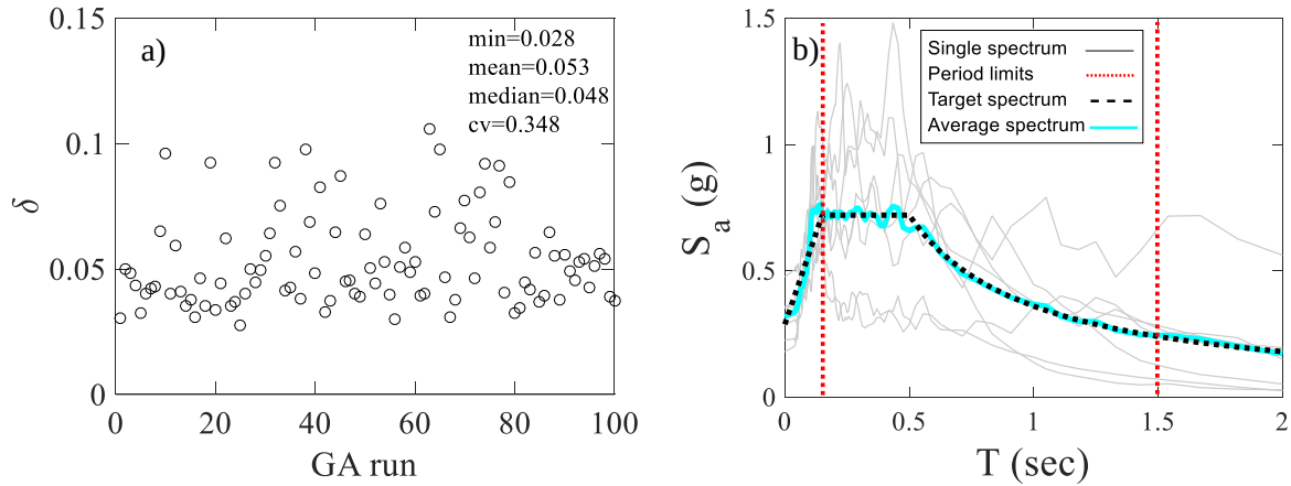
Figure 2. Single-objective ground motion selections using the GA algorithms. a) \delta values obtained from different GA runs; b) Spectra of the selected ground motion set
