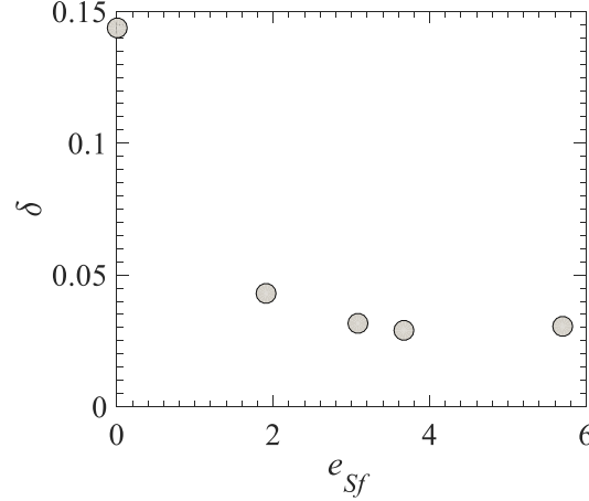
Figure 7. \delta versus e_{sf} Pareto-front optimal solutions
