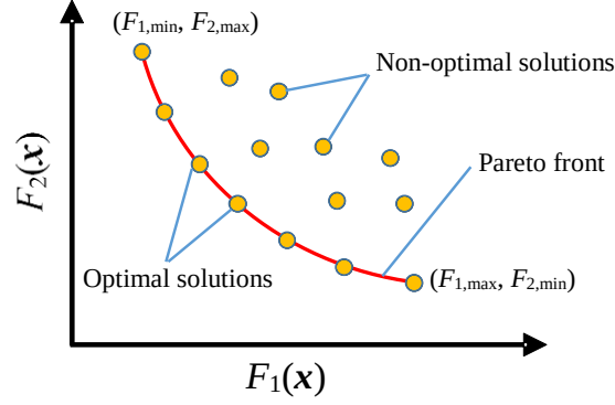
Figure 1. Pareto-optimal solutions
