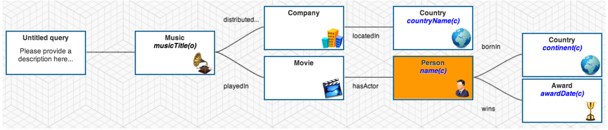
Fig. 13. A complex query formulated by casual users.
