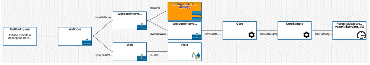
Fig. 11. A complex query formulated by Statoil's domain experts.
