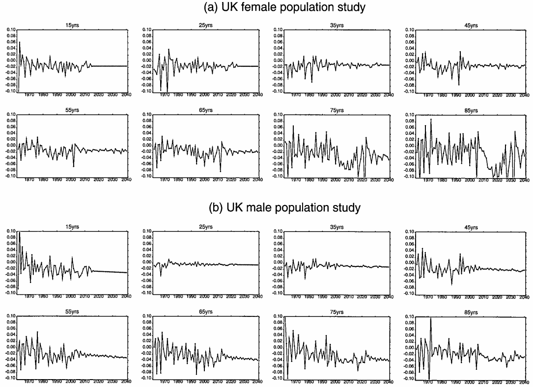
Fig. 8. Secular trends in \frac{1}{\mu_{xt}} \frac{\partial \mu_{xt}}{\partial t} for selected ages x , incorporating model M projections- (a) UK female population study; (b) UK male population study
