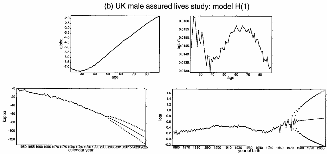
Fig. 5. UK male assured lives study, parameter estimates- (a) model M; (b) model H 1
