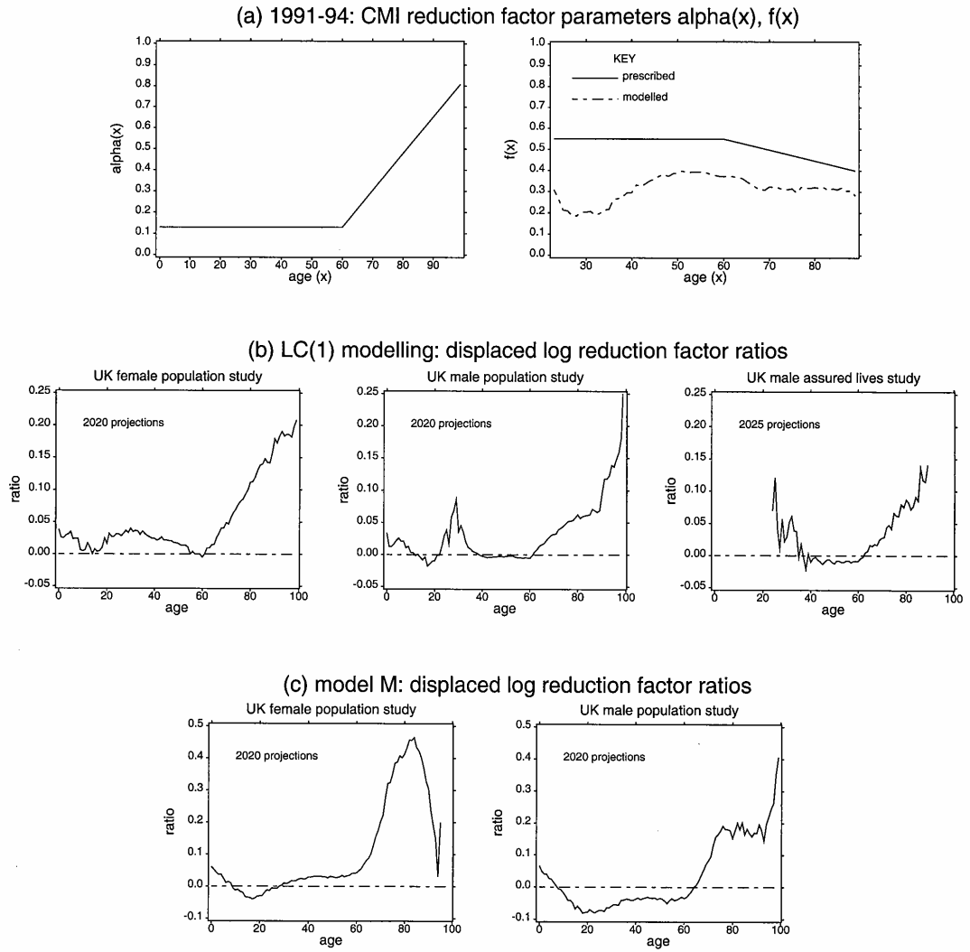
Fig. 7. (a) UK male assured lives study: prescribed asymptotes \alpha(x) , matching f(x) profiles. Displaced ratio 1 - \log \dot{F}_\alpha / \log \dot{F} age profiles, fixed period (b) model LC(1); (c) model M
