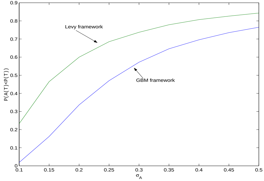
Figure 3: Default probabilities in the two market paradigm presented in the paper and their sensitivity to the reference portfolio volatility.
