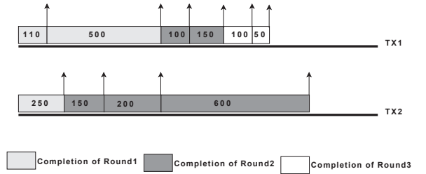
Fig. 12. Overlapping of all the three rounds in MCDRR Scheduling
